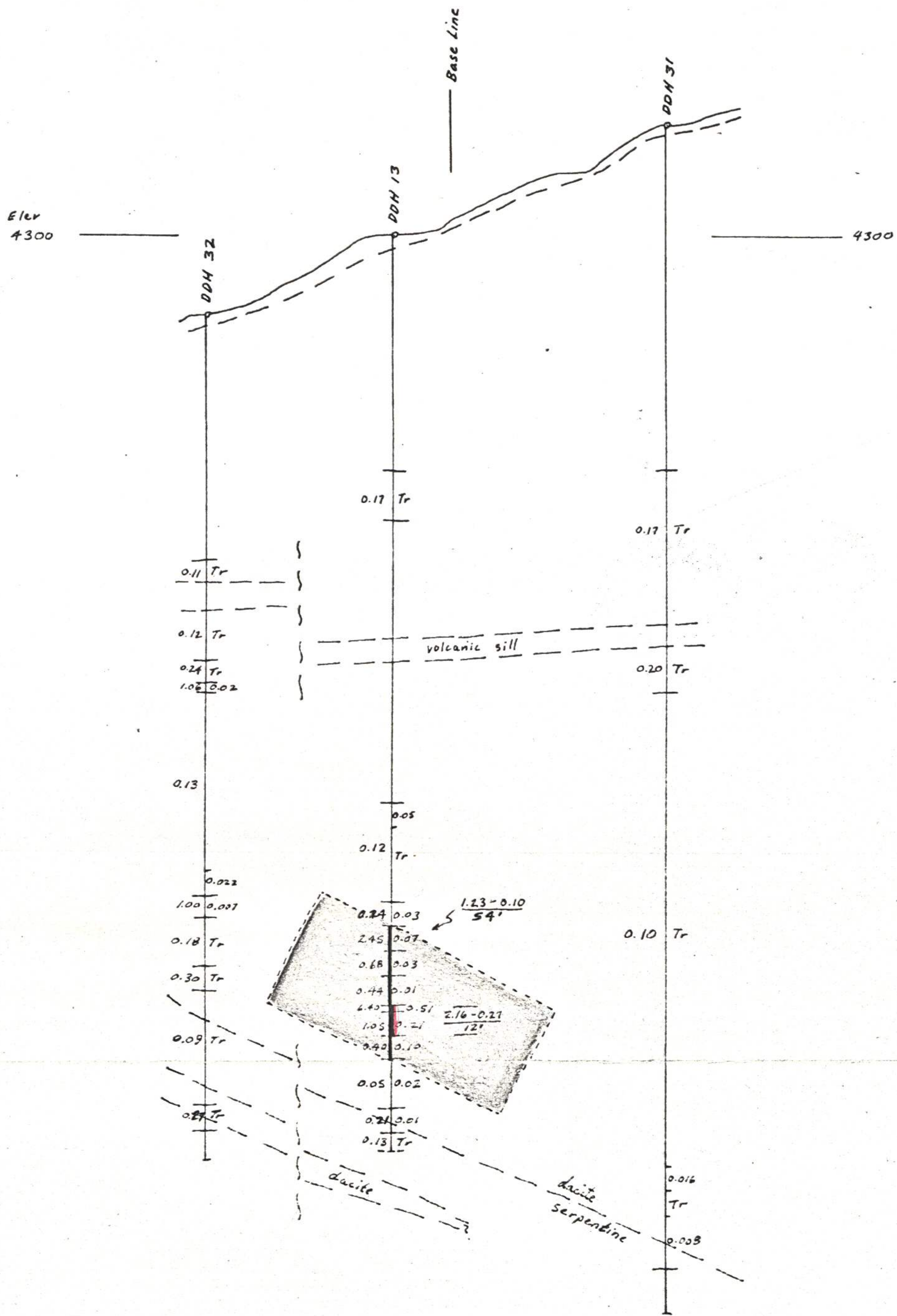
SECTION 18+29N LOOKING NORTHWEST 1" = 50'
