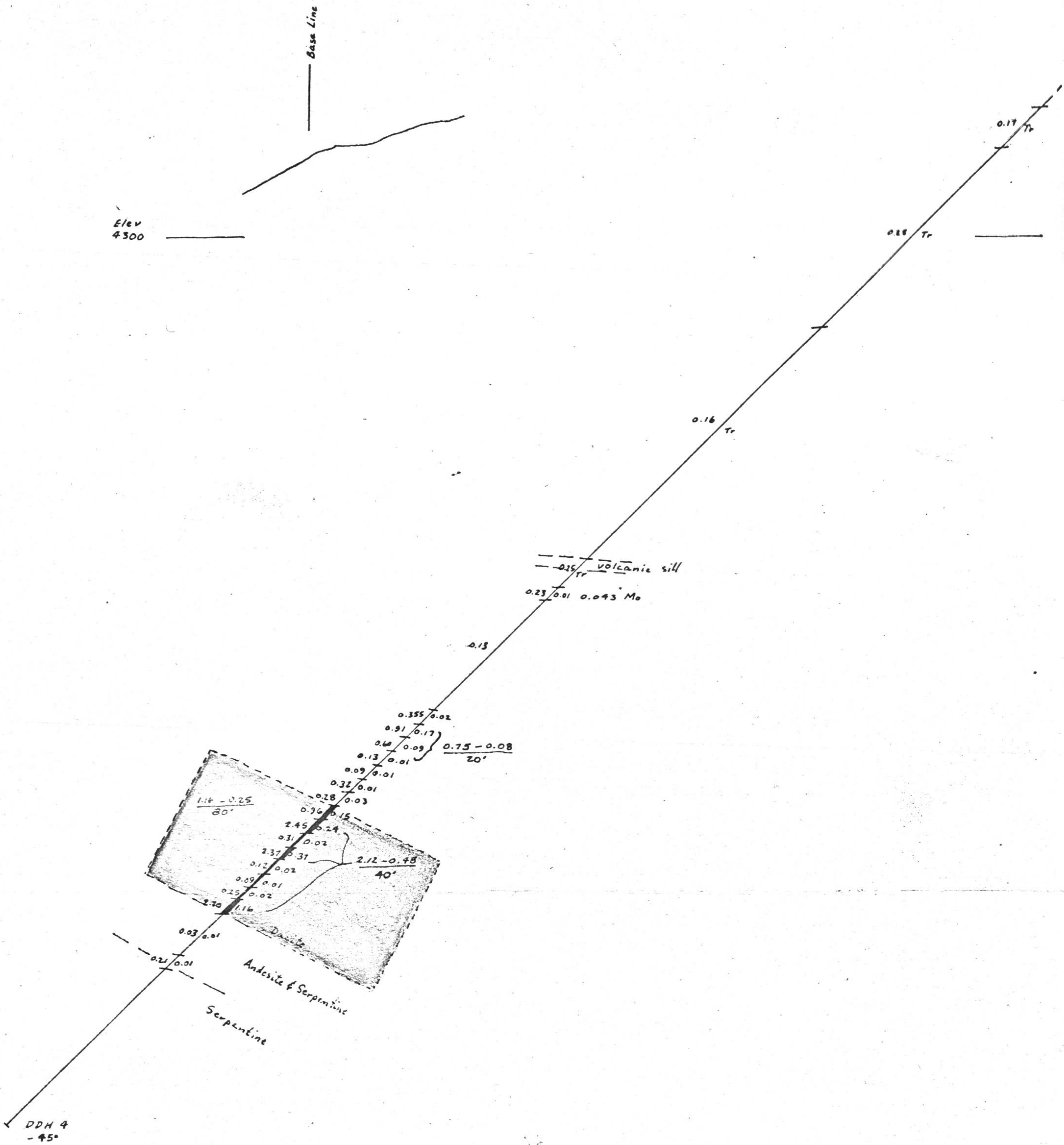
SECTION 16+20N LOOKING NORTHWEST 1" = 50'
