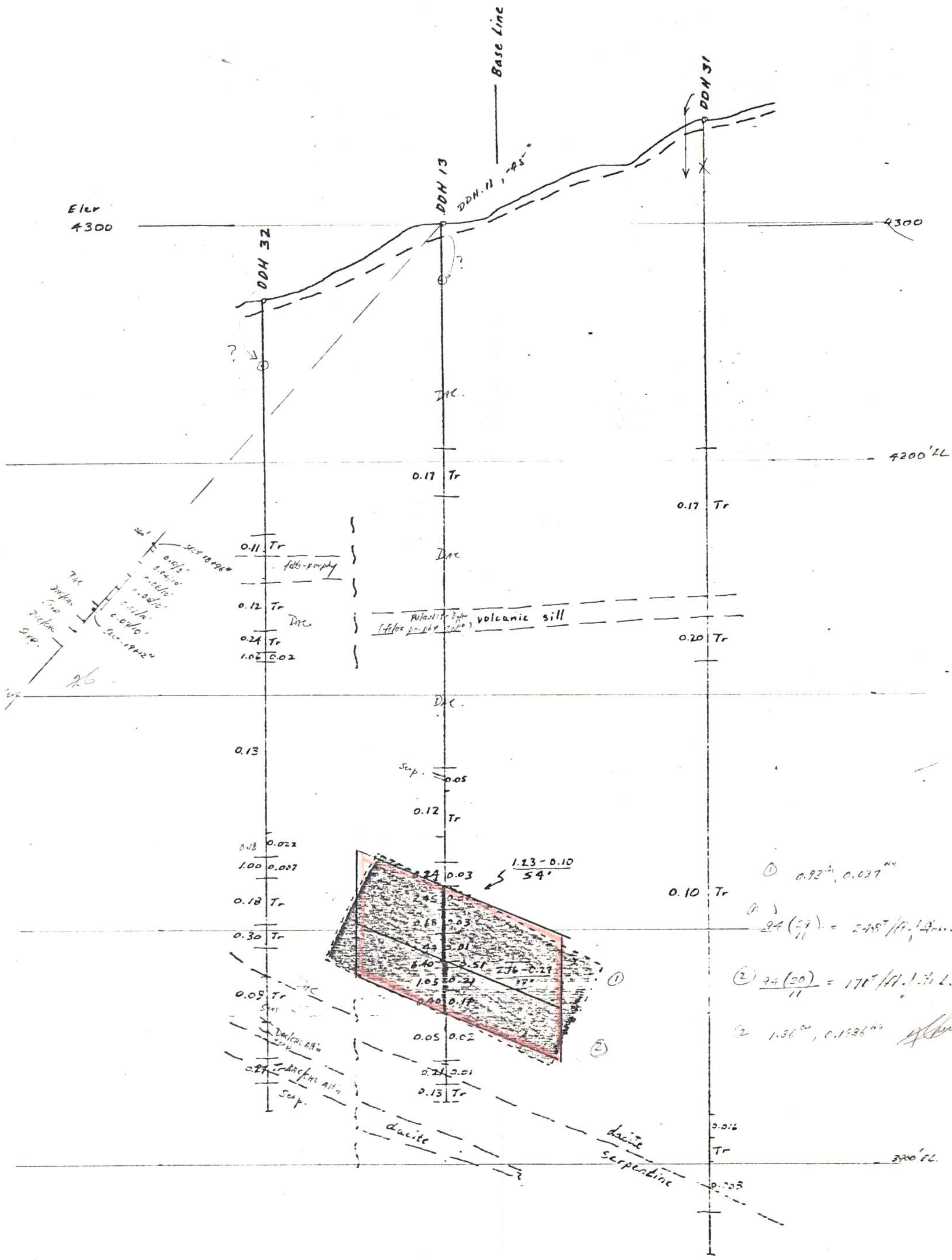
15 SECTION 18+35N LOOKING NORTHWEST 1" = 50'
