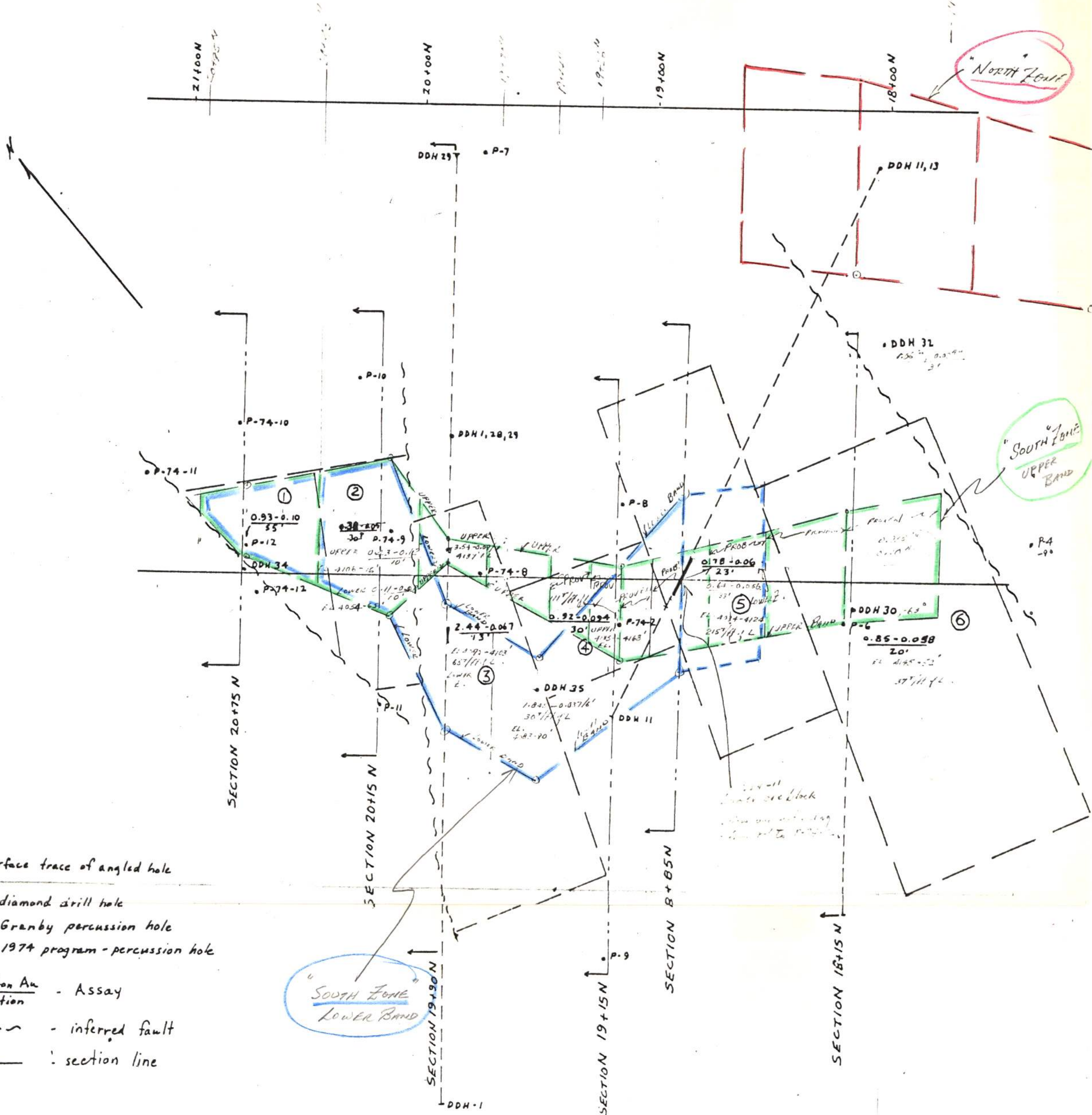
Atlenian Resources Ltd. GREENWOOD GOLD-COPPER PROPERTY SURFACE PLAN MAIN ZONE - NEAR SURFACE SECTION 1" = 50 ft.
