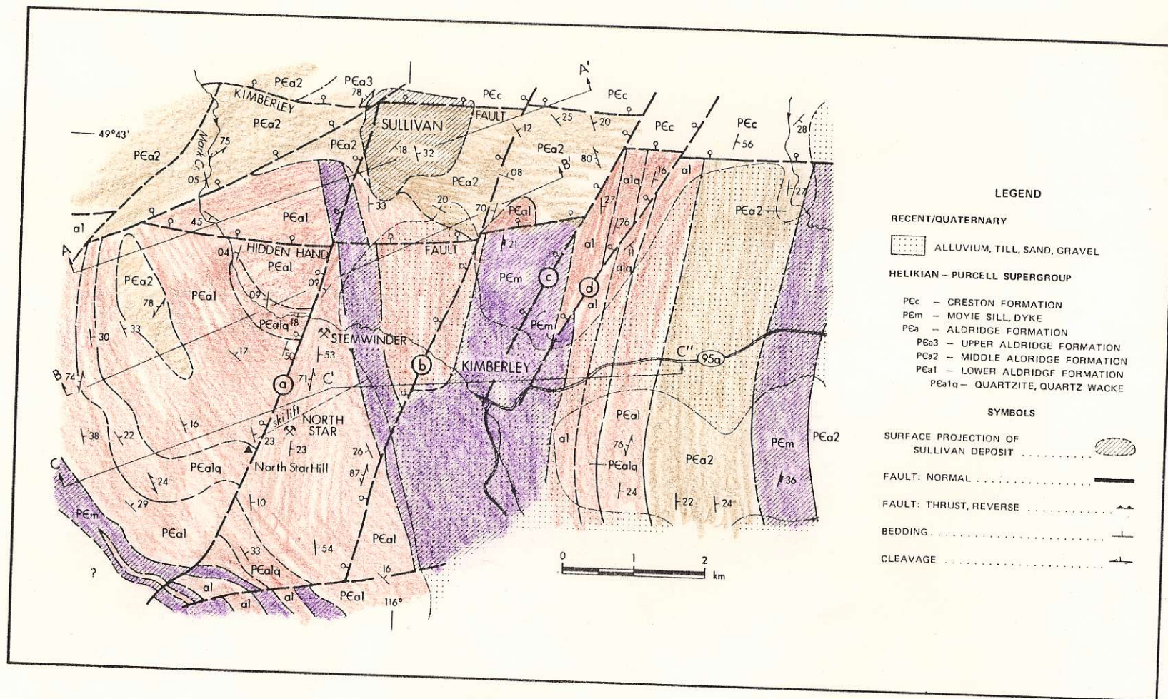
Figure 6. Geology in the vicinity of the Sullivan deposit, Kimberley.
