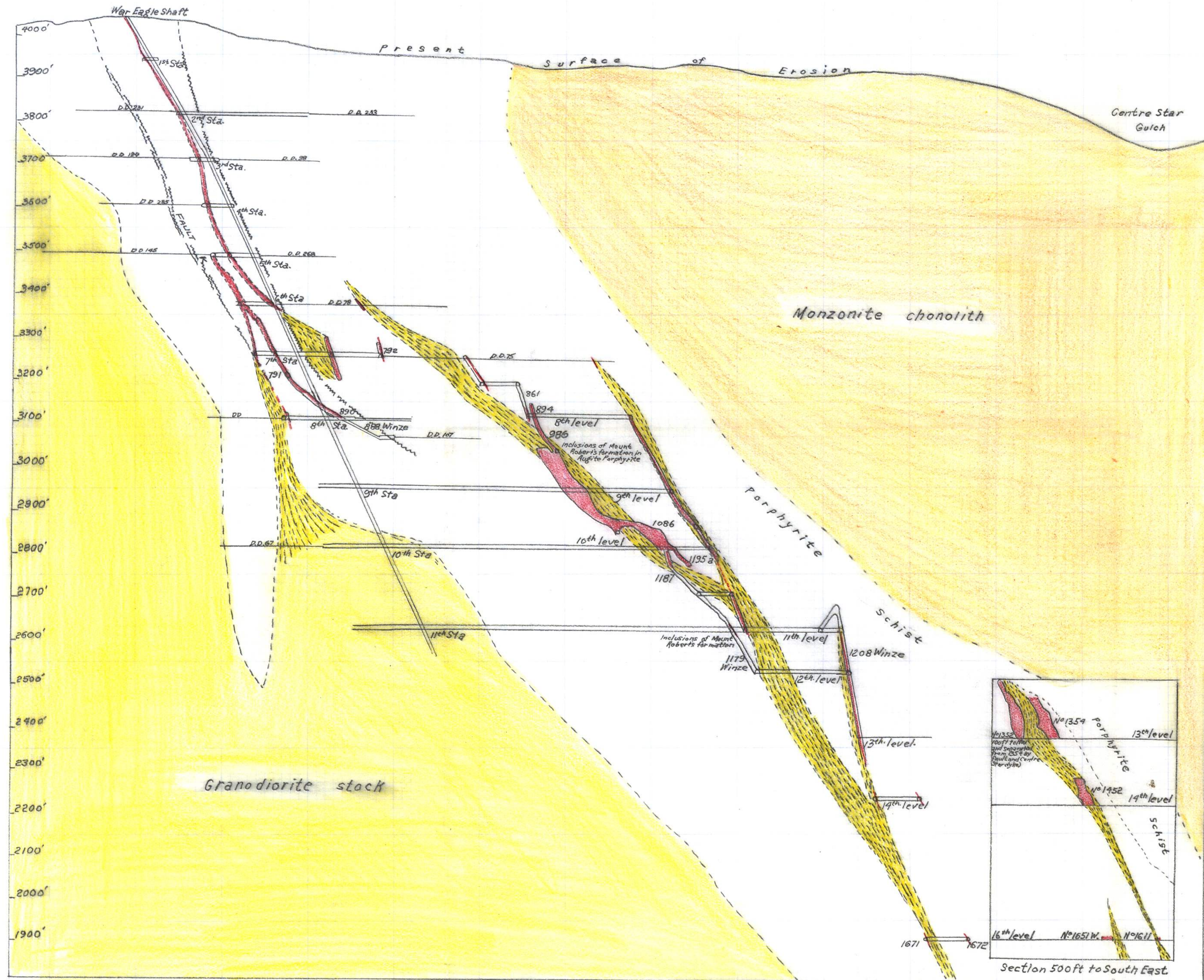
Vertical Section AB through War Eagle Mine, Rossland, B.C.
