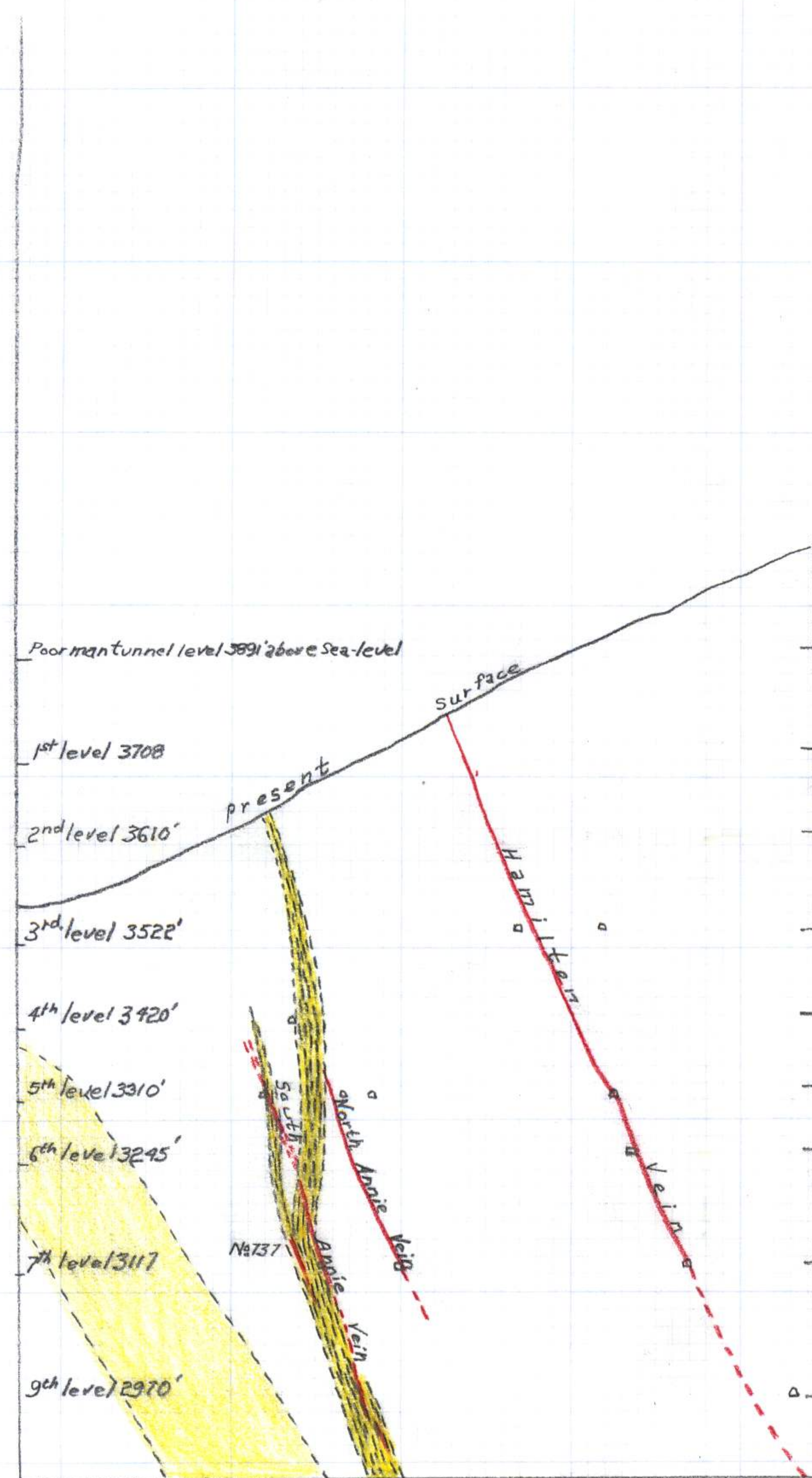
Vertical Section E-F through Annie and Hamilton Veins Josie Mine
