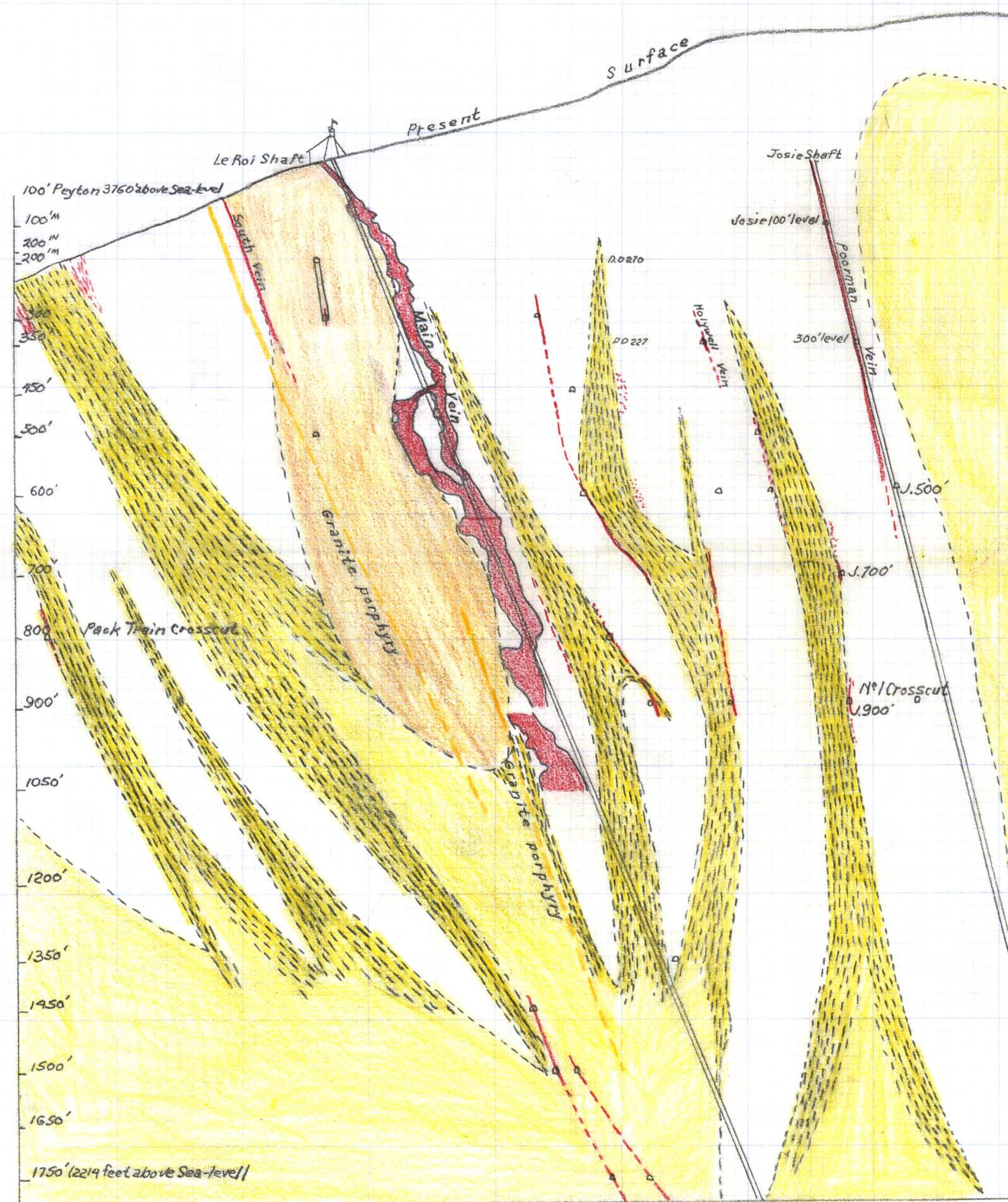
Vertical Section C-D through Le Roi Mine 125 feet east of Main Shaft
