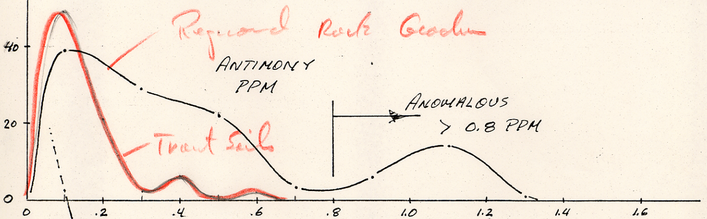
Fig 7 Comparison of the Geochemistry of Trout Sails with that of Regional Eocene Volcanic Rocks.
