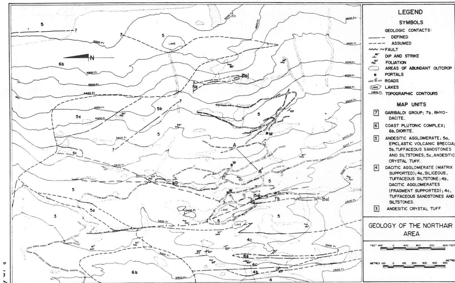
Figure 32. Detailed geological map of a part of Callaghan Creek pendant including mineral deposits of Northhair Mines Ltd. Portals to the main deposits are labelled: M – Manifold zone, W – Warman zone, and D – Discovery zone. A–A 1 is the location of a cross-section through the Warman zone, shown in Figure 35.
