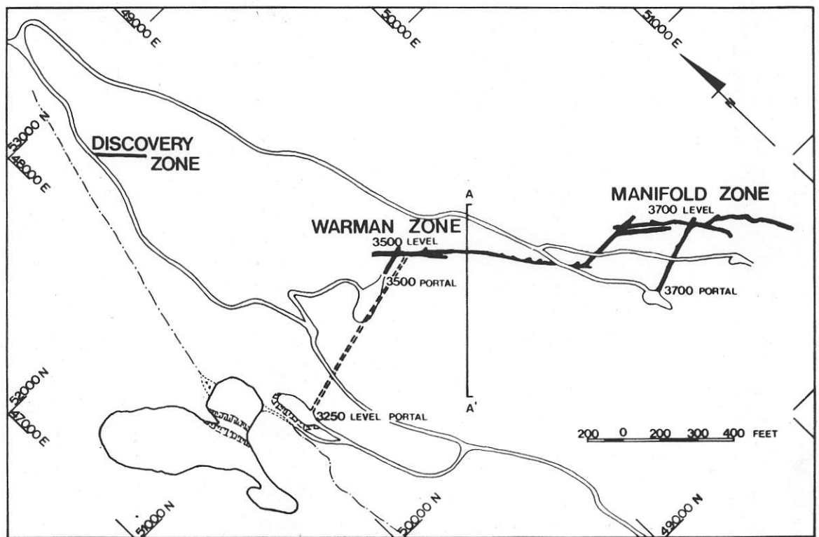
Figure 34. Generalized plan of underground haulage levels showing relative locations of three principal ore zones. A-A 1 is location of the cross-section of Figure 35 (modified from Dickson and McLeod, 1975).
