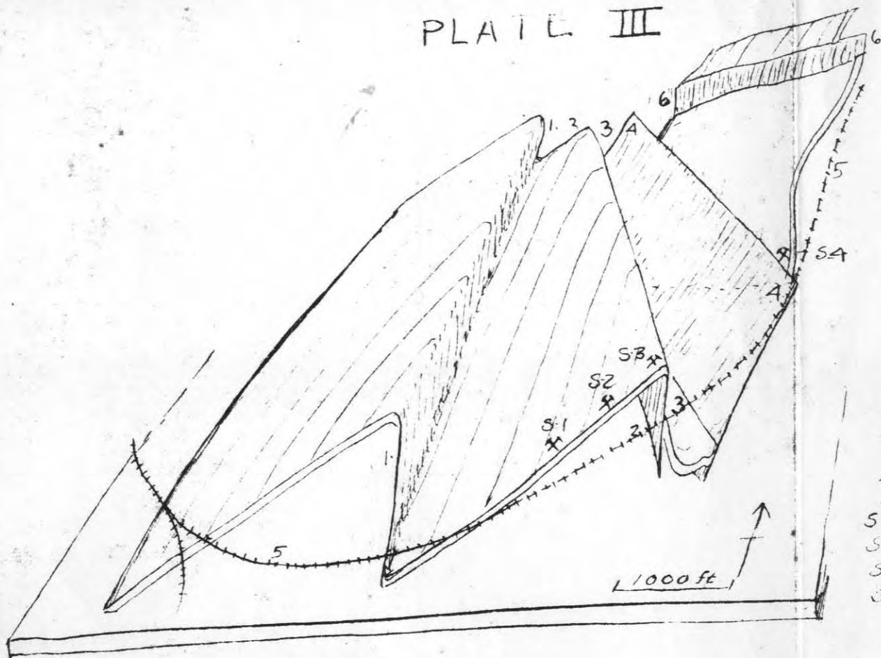
SHAPE OF SUNNYSIDE LIMESTONE IN NICKEL PLATE AREA. (somewhat simplified)
