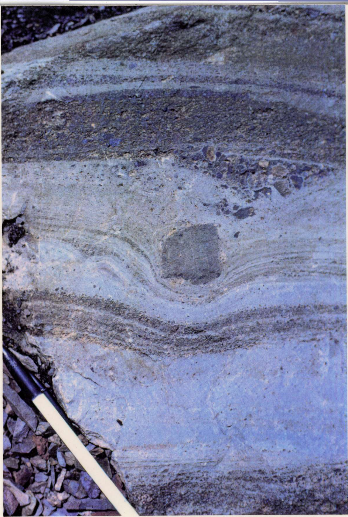
Ballistically emplaced clast, Betty Creek Formation
