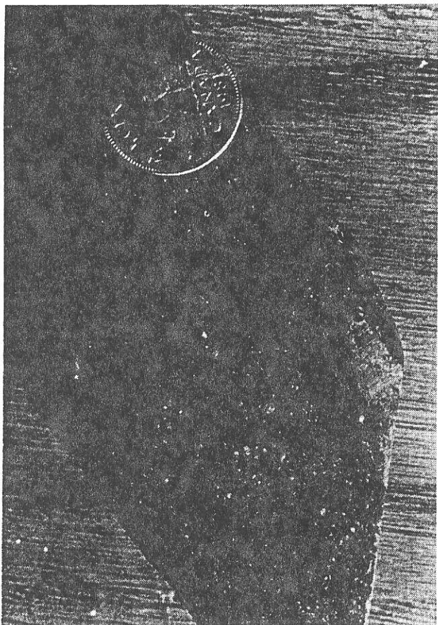
Plate B-14-4. Banded sphalerite, tetrahedrite, boulangerite and bournonite in contact unit pyritic mudstone, southern 21B deposit, Eskay Creek (DDH CA89-87: 97 m).
