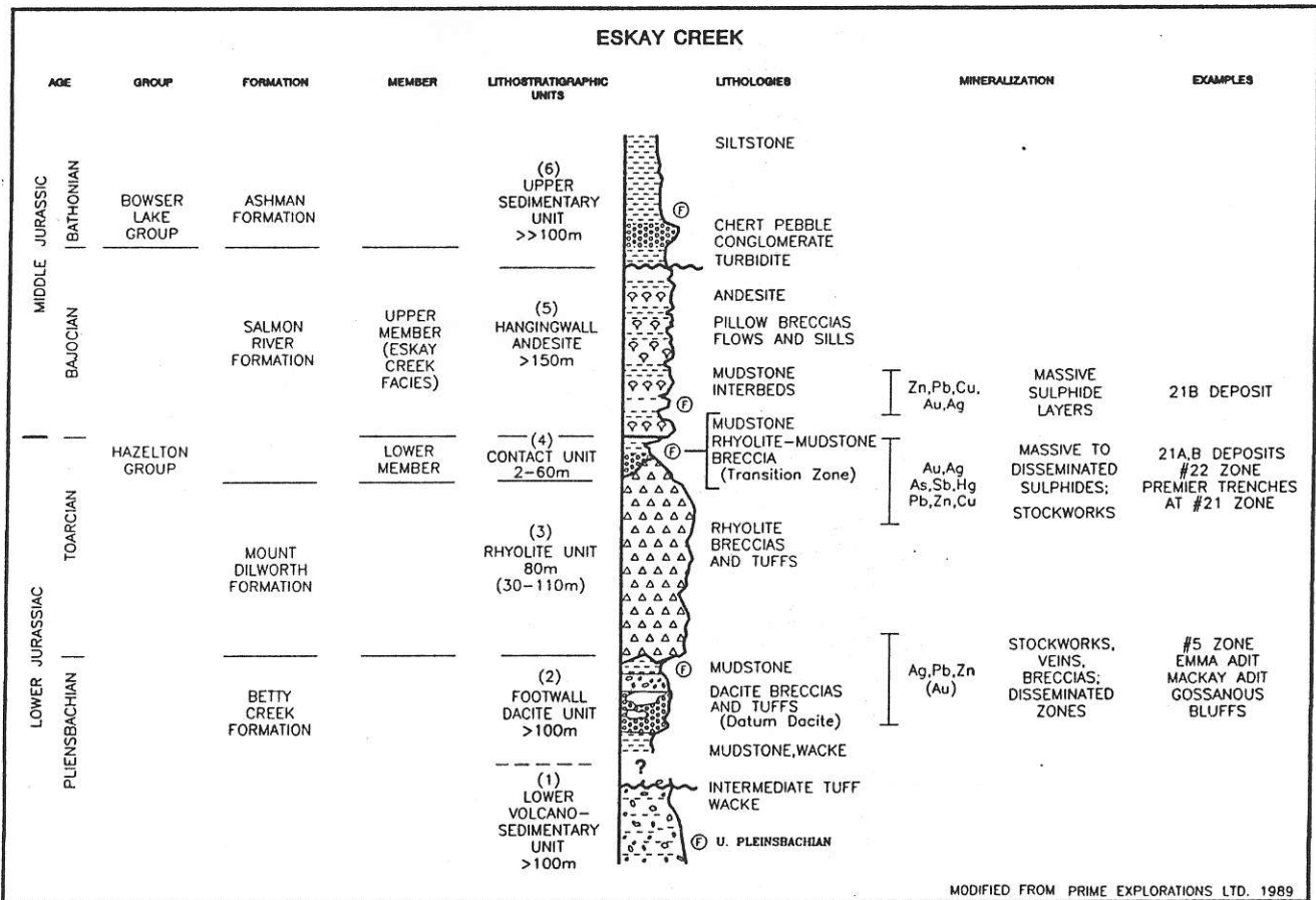
Figure B-14-4. Stratigraphy and mineralization, Eskay Creek.
