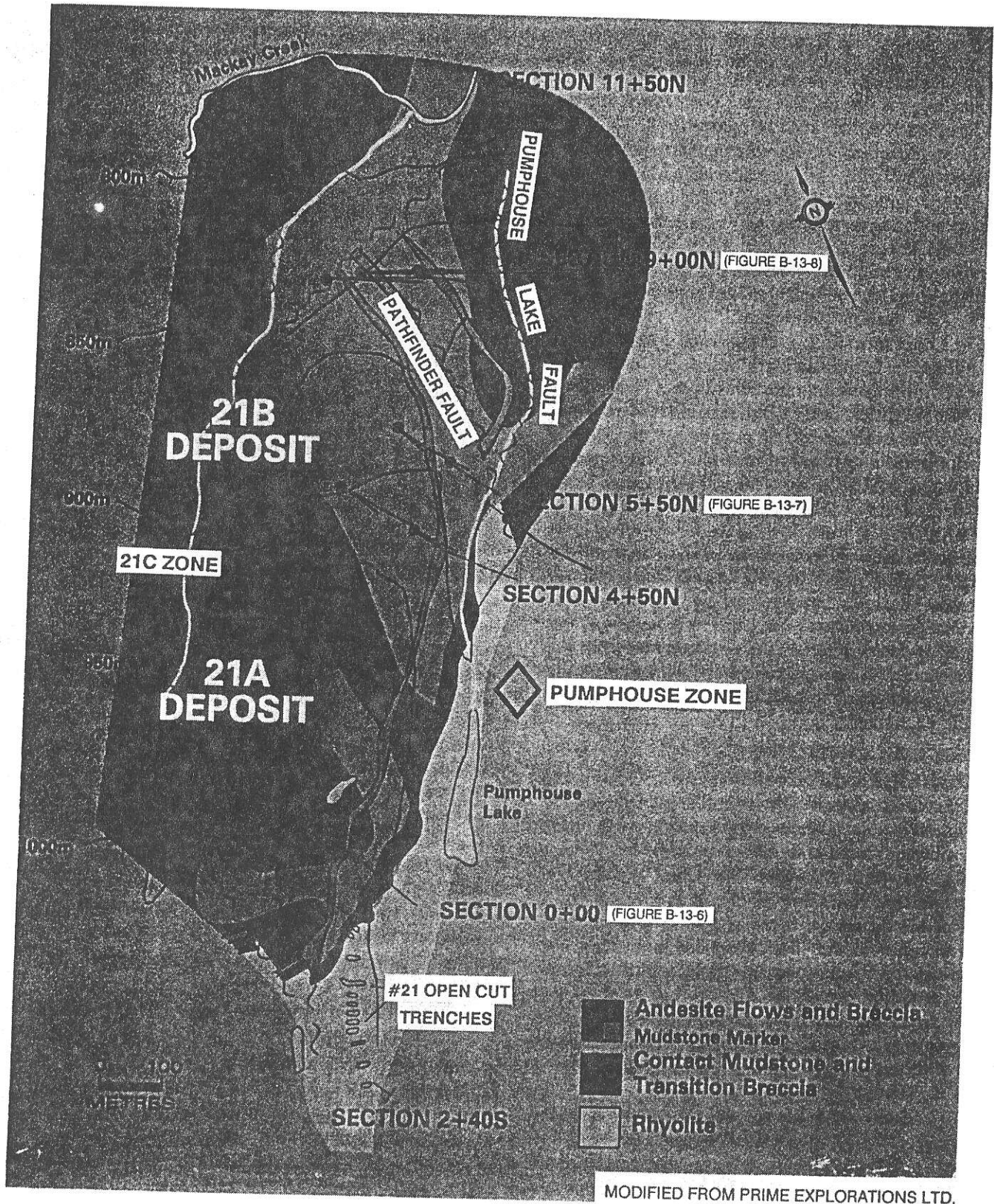
Figure B-14-5. Deposit plan, #21 zone, Eskay Creek.
