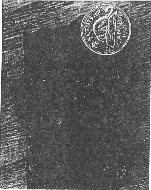
Plate B-14-6. Sulphide-rich vein with coarse-grained galena and zoned sphalerite, northern 21B deposit, Eskay Creek (DDH CA89-109: 90.5 m).
