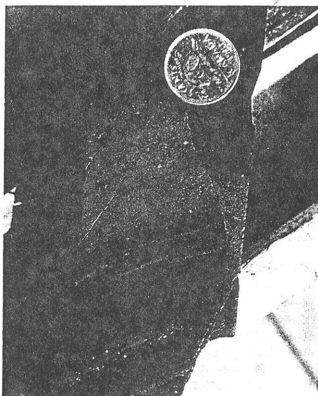
Plate B-14-3. Sulphide layers in contact unit mudstone, southern 21B deposit, Eskay Creek (DDH CA89-68: 101 m).
