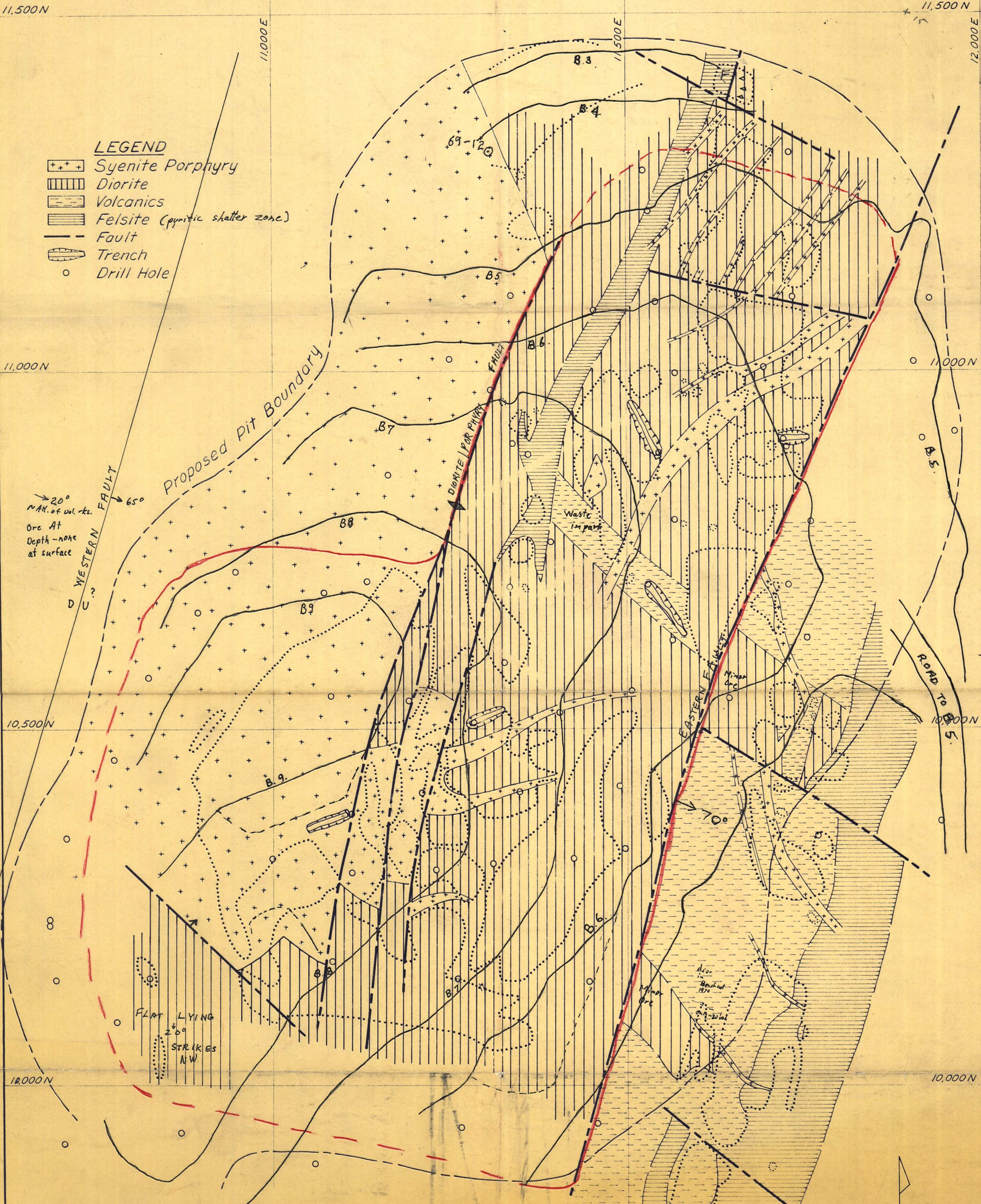
Figure 2 GRANISLE SURFACE GEOLOGY PIT AREA
