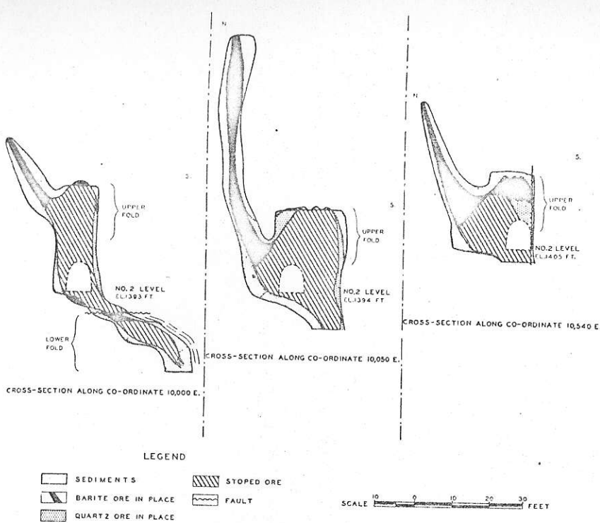
Figure 7.—North-south cross-sections through stopes on North ore-body, showing details of drag-fold in this ore-body.
