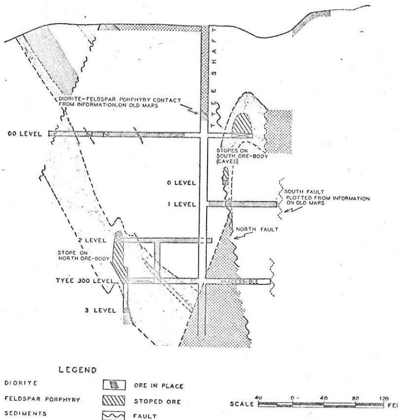
Figure 5.—North-south cross-section through the Tye shaft showing stopes on the North and South ore-bodies. Information not found in those workings in the plane of sections has been compiled from diamond-drill hole data and from nearby cross-sections.
