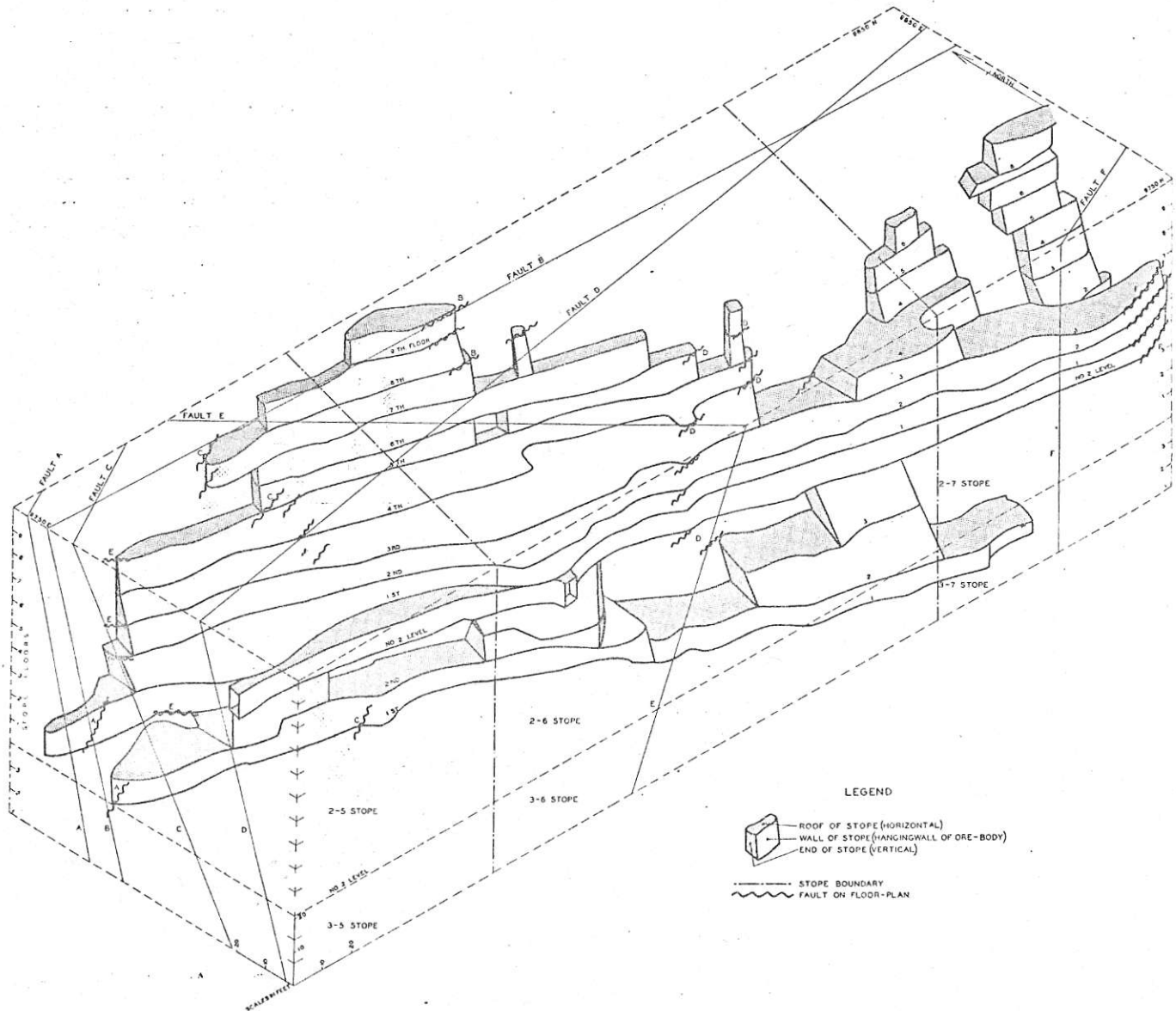
Figure 6.—Block diagram or isometric projection of a block of stopes on the North ore-body. The diagram represents the ore as a solid body, contoured at each stope floor. The projection begins at 3rd floor below No. 2 level and ends at the roof of the stope nine floors above the level. Compiled from geology mapped on floor-plans and from geology on several cross-sections.
