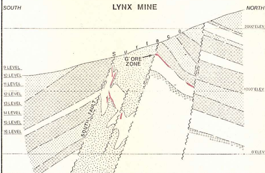
CROSS-SECTION 60+00 E. LOOKING WEST
