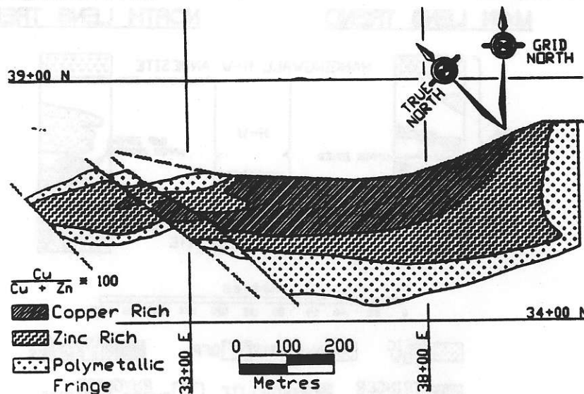
FIG 5 - H-W main lens metal zoning plan.
