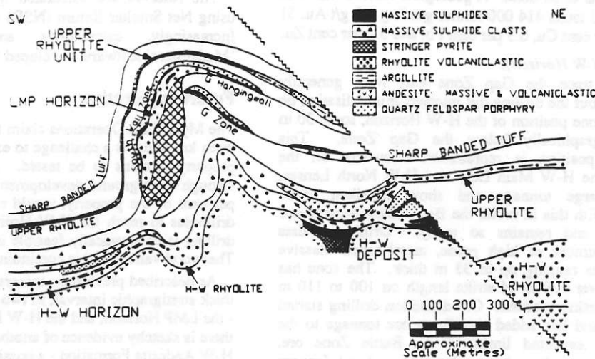
FIG 7 - Mine sequence composite cross section.
