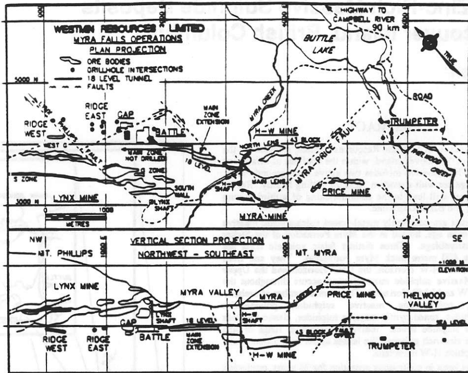
FIG 2 - Plan projection and vertical section projection.
