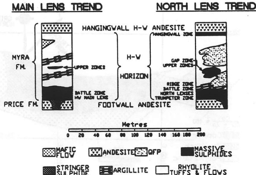
FIG 4 - Stratigraphic column H-W Horizon.
