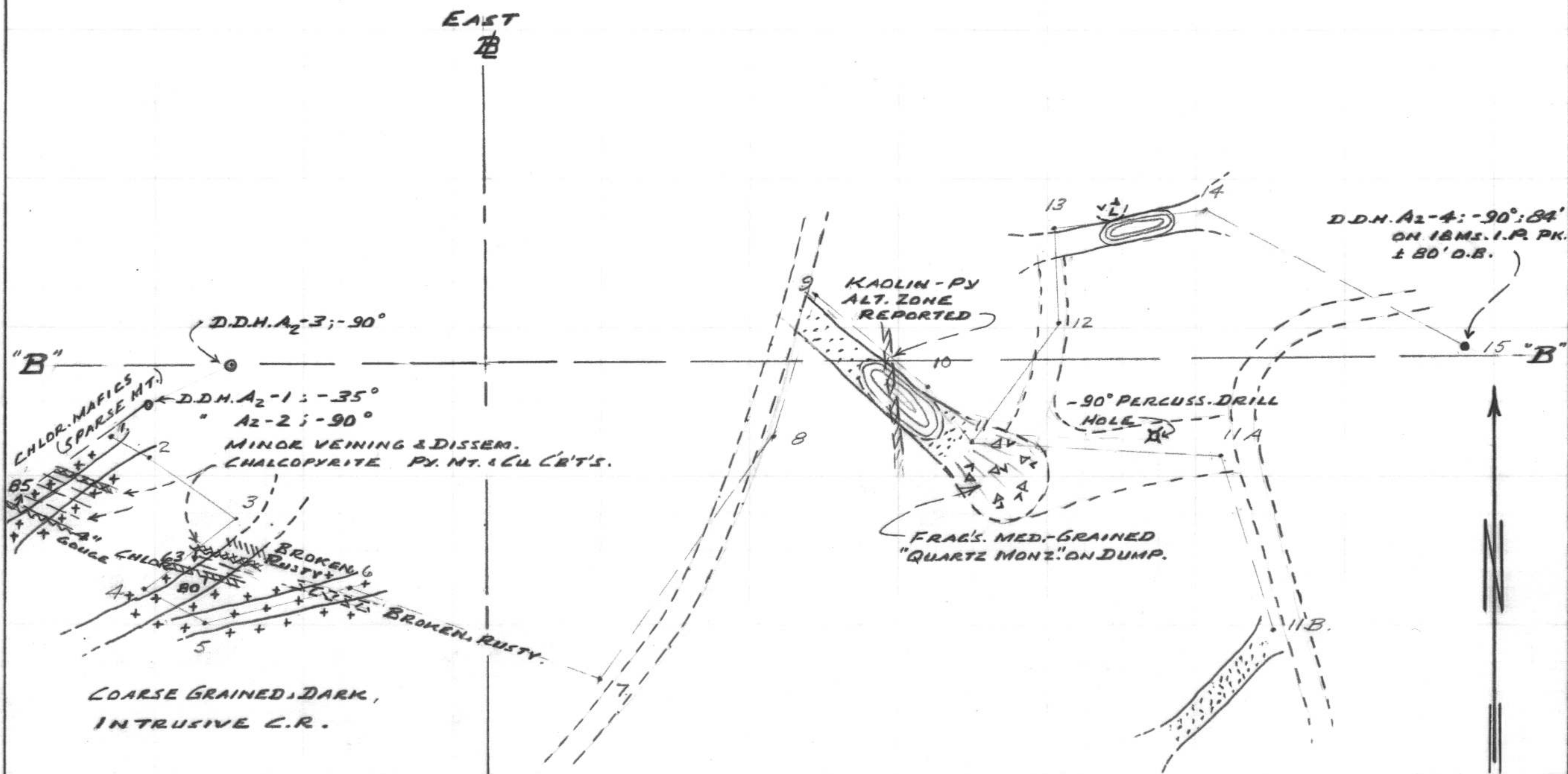
FIG. 3 A-2 ZONE GEOLOGY, TRENCHES, DRILL HOLES SCALE: 1" = 100' MAY, 1968. MAMIT LAKE MINING LTD. W.M. SHARP, P. ENG. LEGEND: [Symbol] DIORITIC / GRANDIORITIC ROCKS [Symbol] FRACTURES: SHEAR, JOINT, RANDOM. [Symbol] CHALCOPYRITE + MAL. PY. & MT. GOSSAN. MINOR CU CB'TS.
