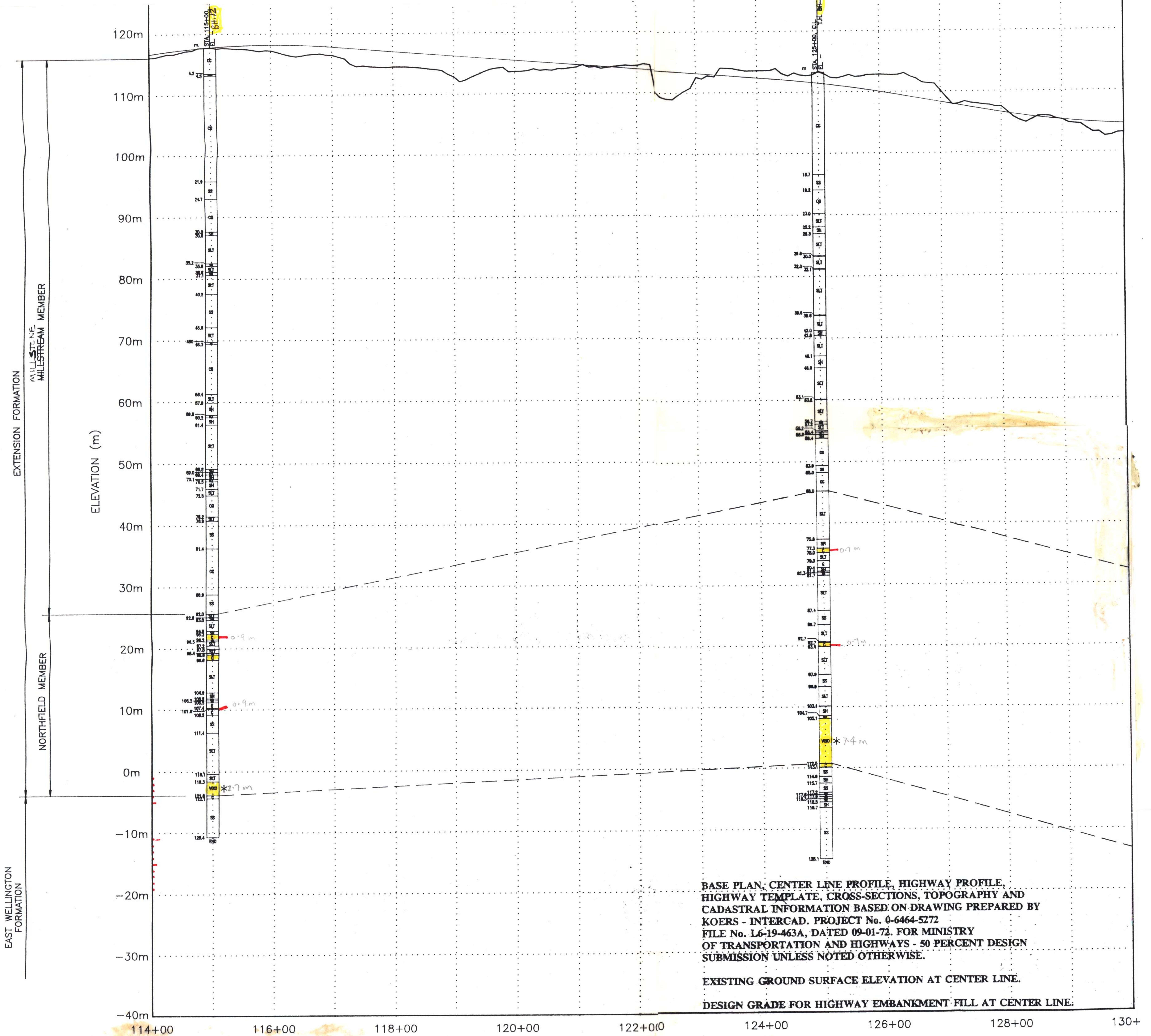
CENTER-LINE PROFILE
