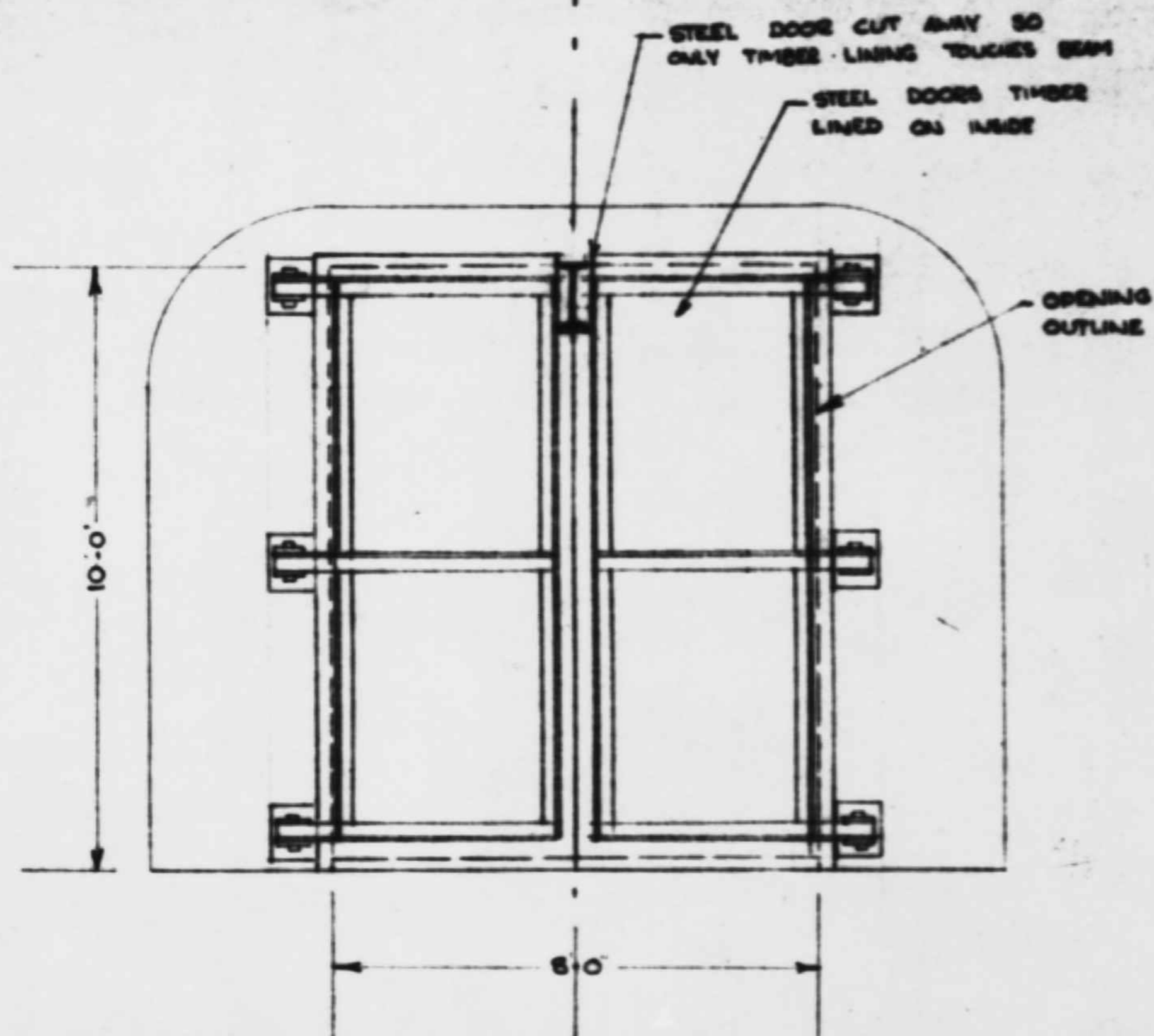
SECTION (SHOWING ARRANGEMENT OF TROLLEY BEAM AND DOOR)
