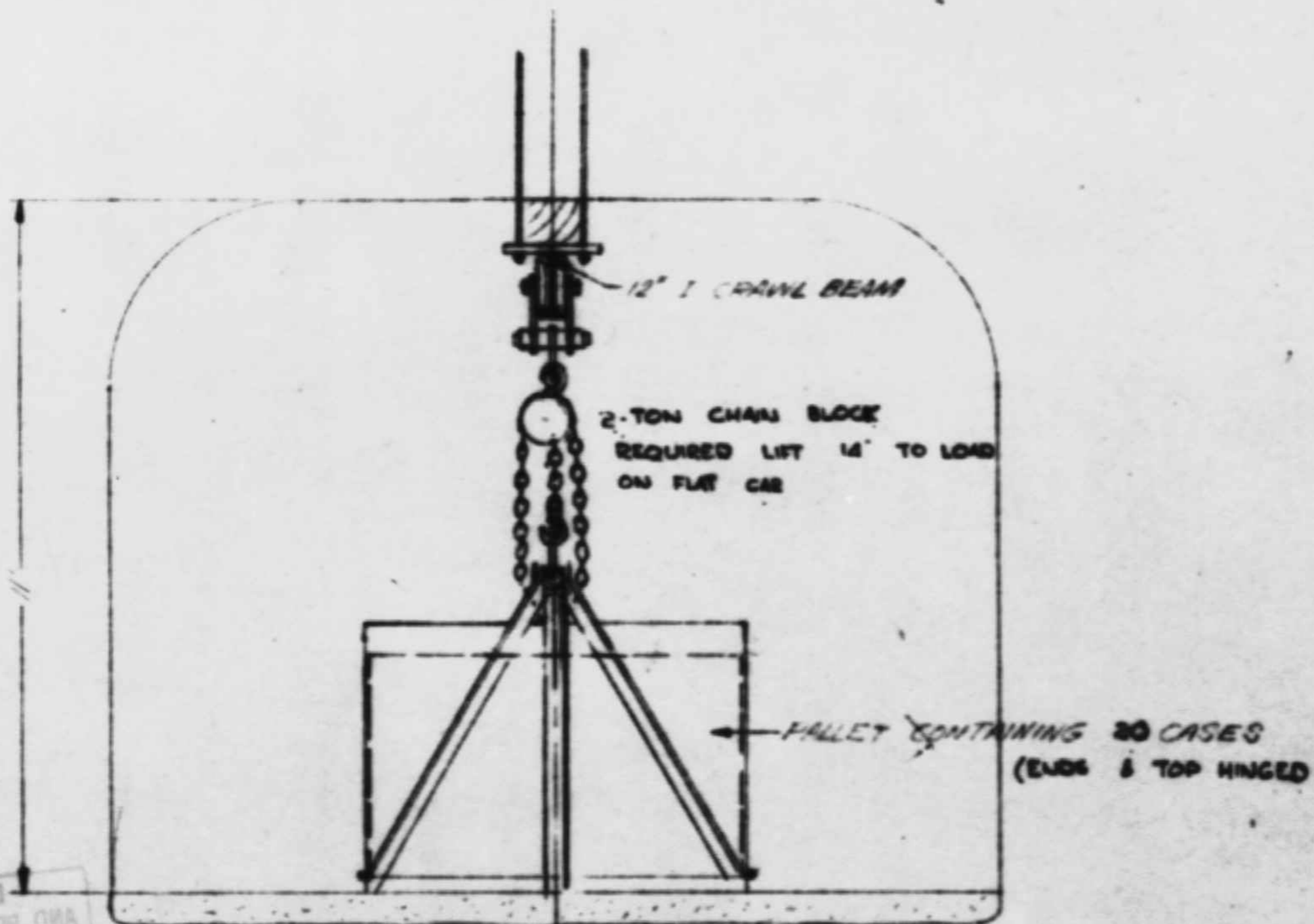
SECTION (SHOWING HANDLING ARRANGEMENT FOR POWDER PALLETS)
