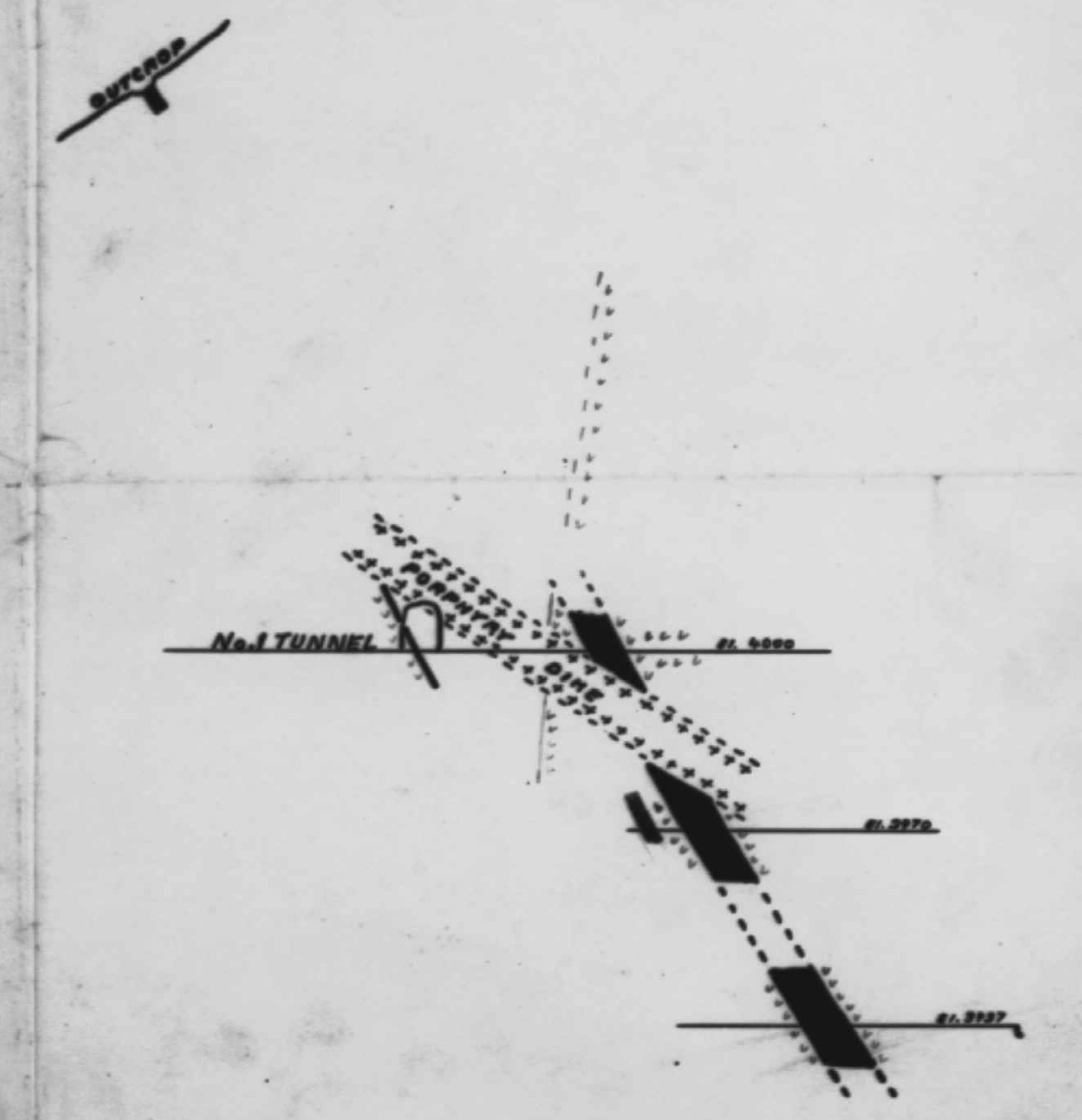
VERTICAL SECTION AT HOLE D+ INTERSECTION AND VEIN OUTCROP Scale - 1 in = 20 feet
