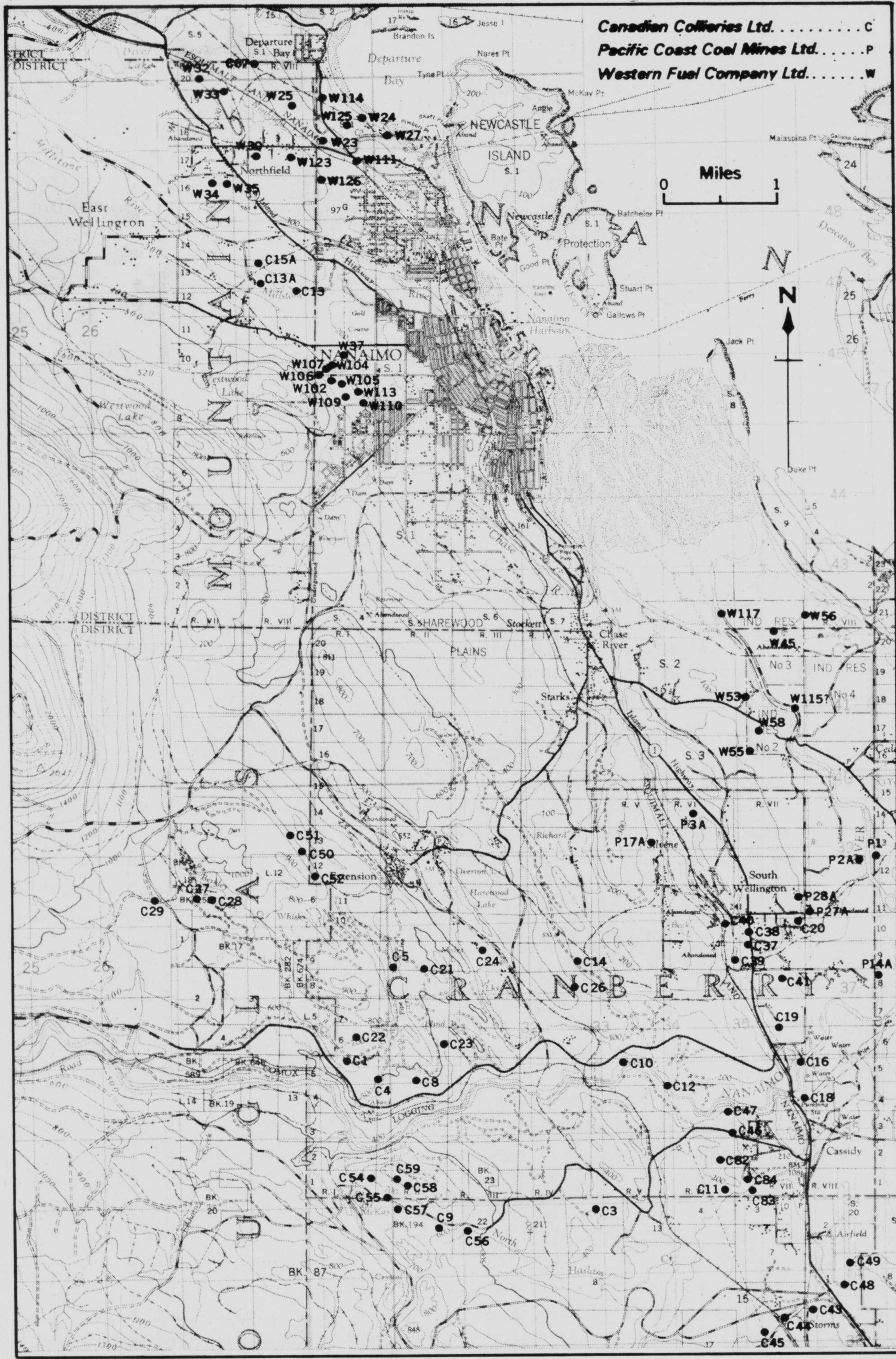
Figure 14. Borehole locations in Nanaimo Field.
