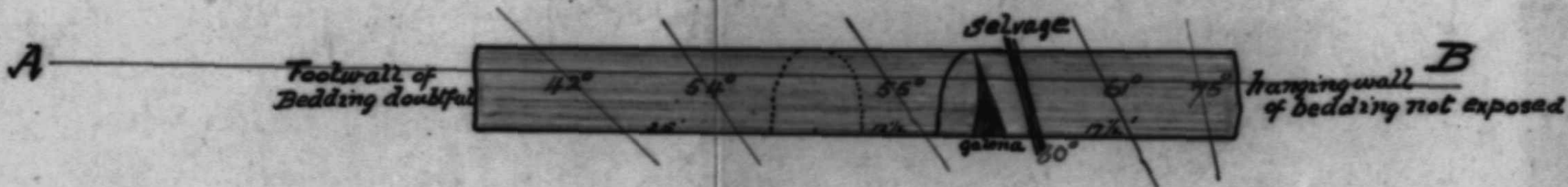
Cross Section on A-B showing variation of dip of bedding due to flexuring or movement of same. Scale 1" = 10'
