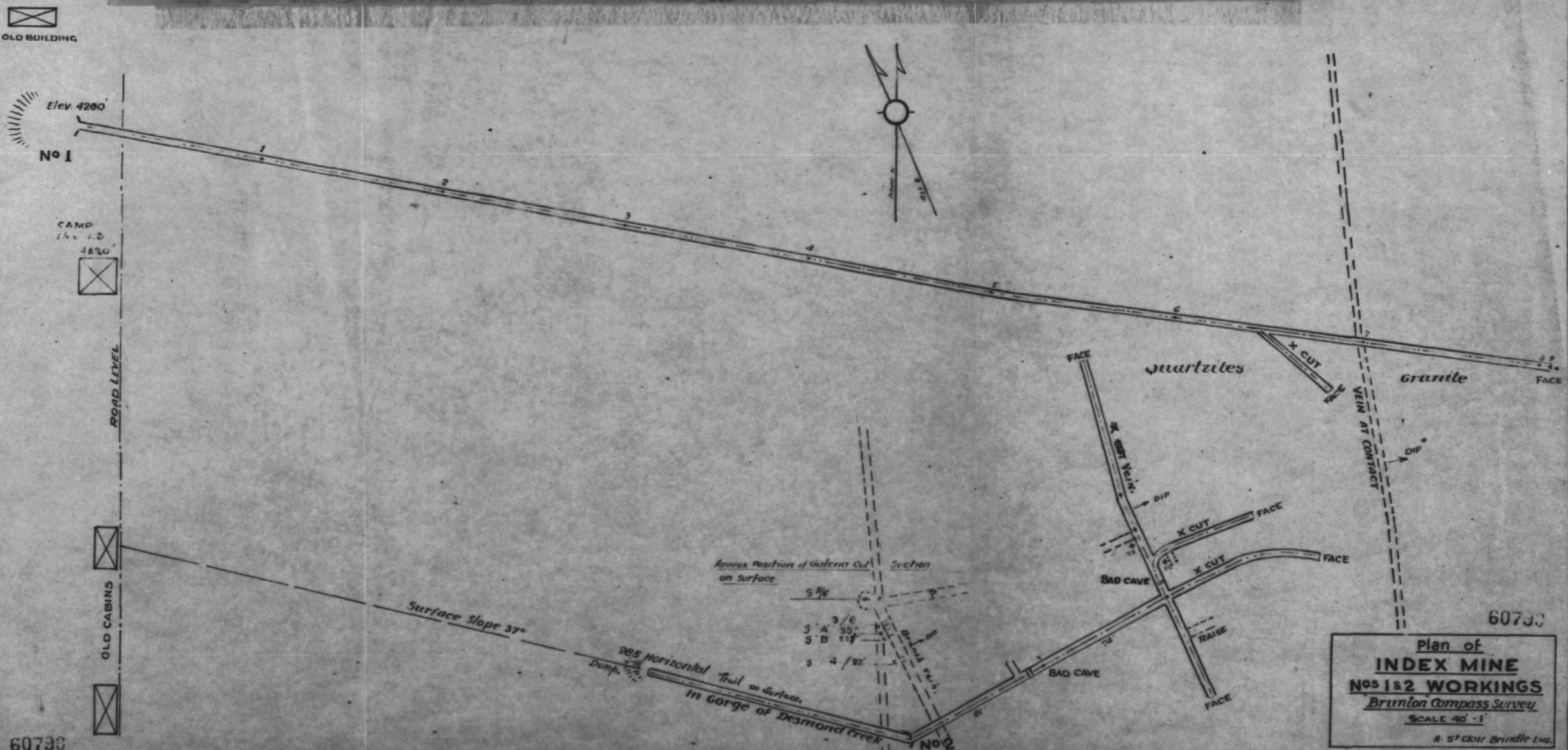
Brunton Compass Survey plan of INDEX FR. ANNEX MINERAL CLAIM WORKINGS ADITS NO. 1 & 2 Situated on South Fork of Kaslo Creek, west Kootenay, B.C. CANADA KASLO SILVER-LEAD CO. Seattle Wash. U.S.A. SCALE 80' = 1" A. Stclair Brunelle Eng.
