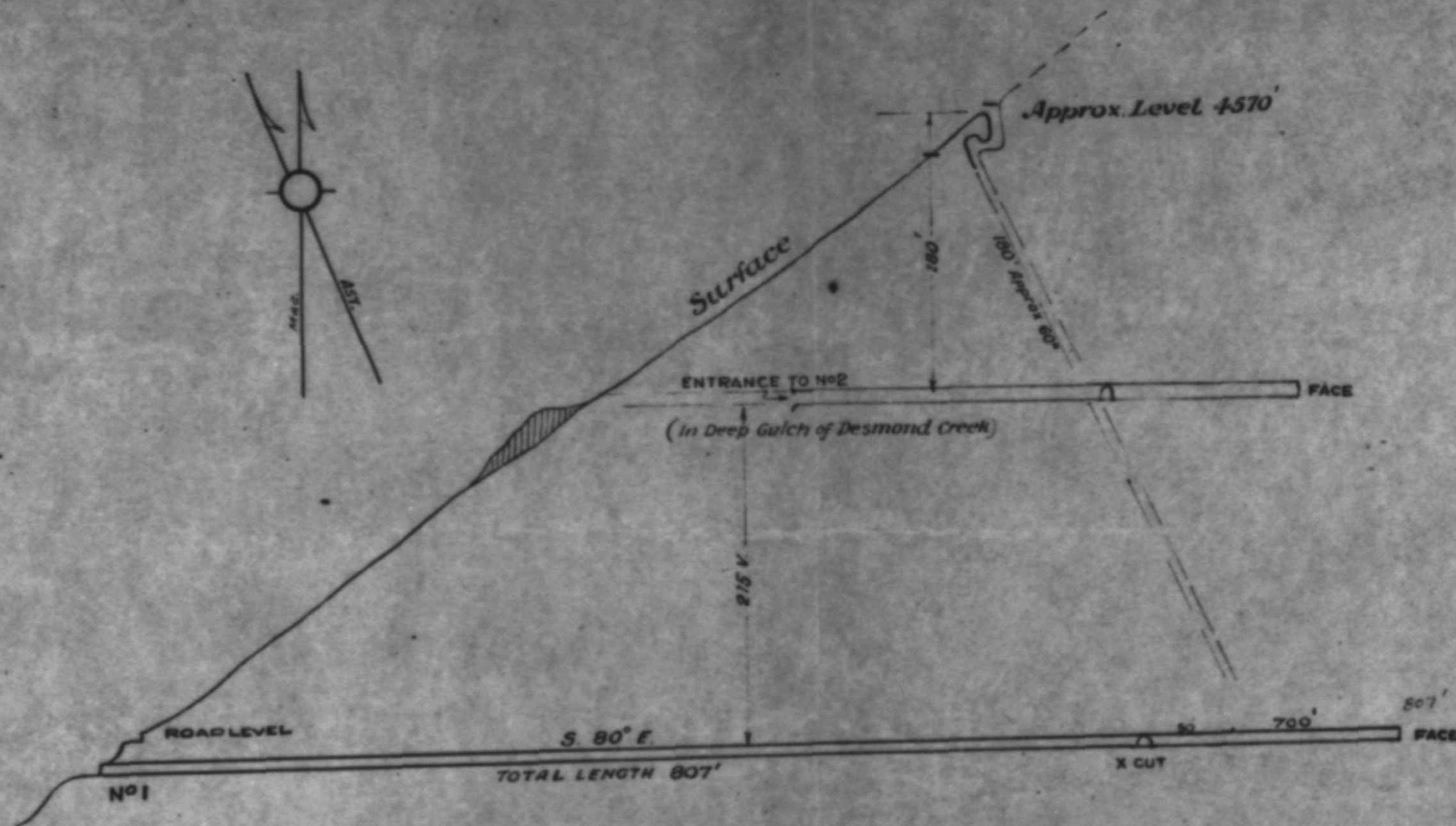
INDEX MINE CROSS SECTION NO. 1 & 2 ADITS (ABOVE CAMP) Brunton Compass Survey SCALE 80' = 1" A. Stclair Brunelle Eng.
