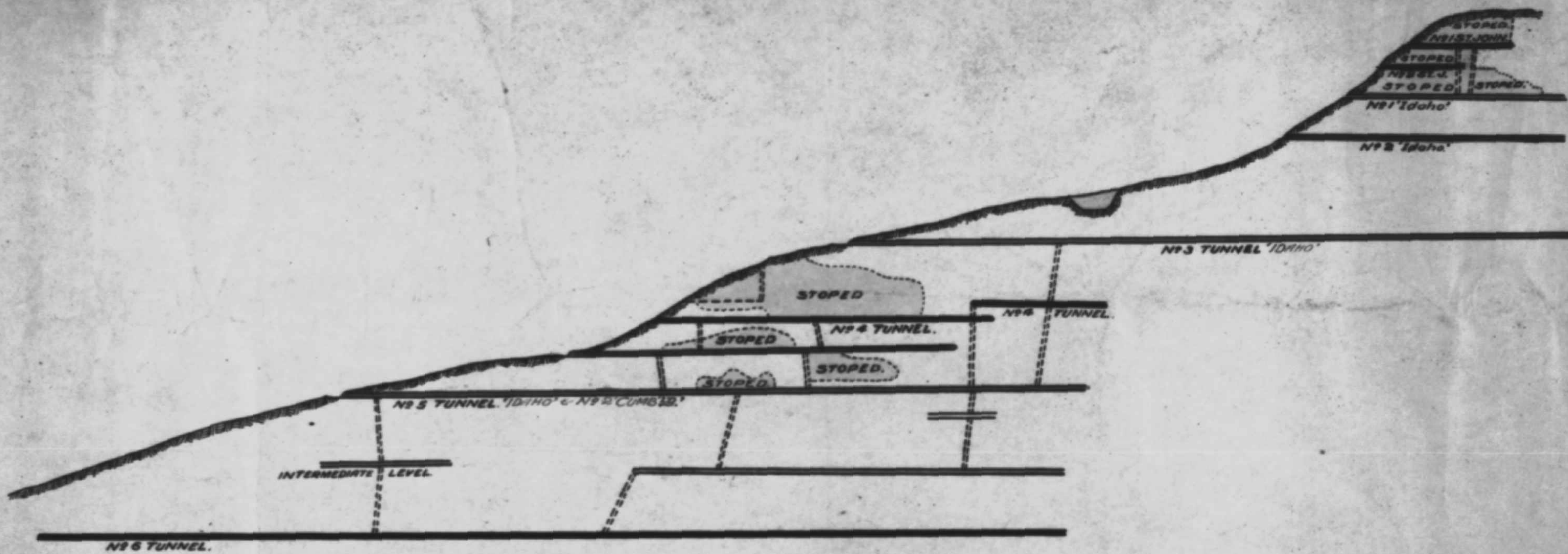
— LONGITUDINAL SECTION. —
