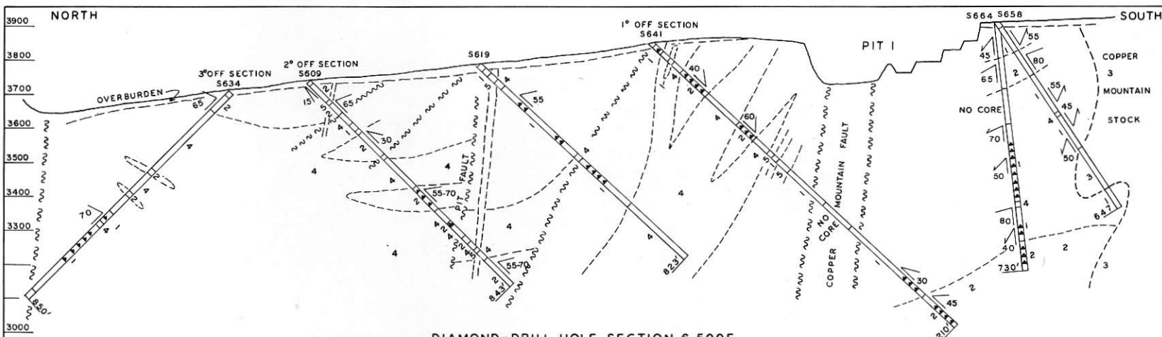
DIAMOND-DRILL HOLE SECTION 6.500E
