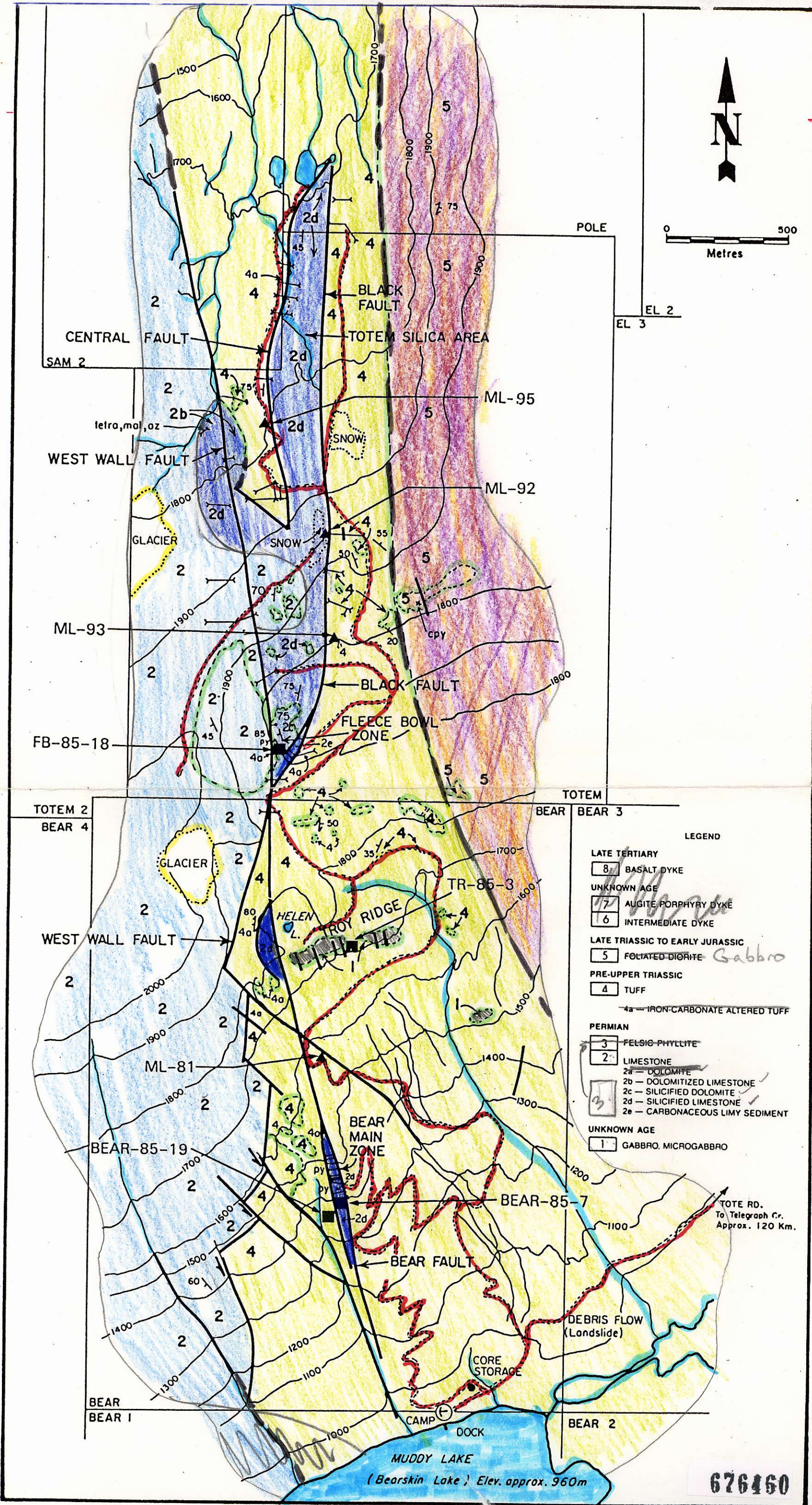
Figure 2-13-1. Location map showing age dates (▲) and chemical analyses (■), Golden Bear property.
