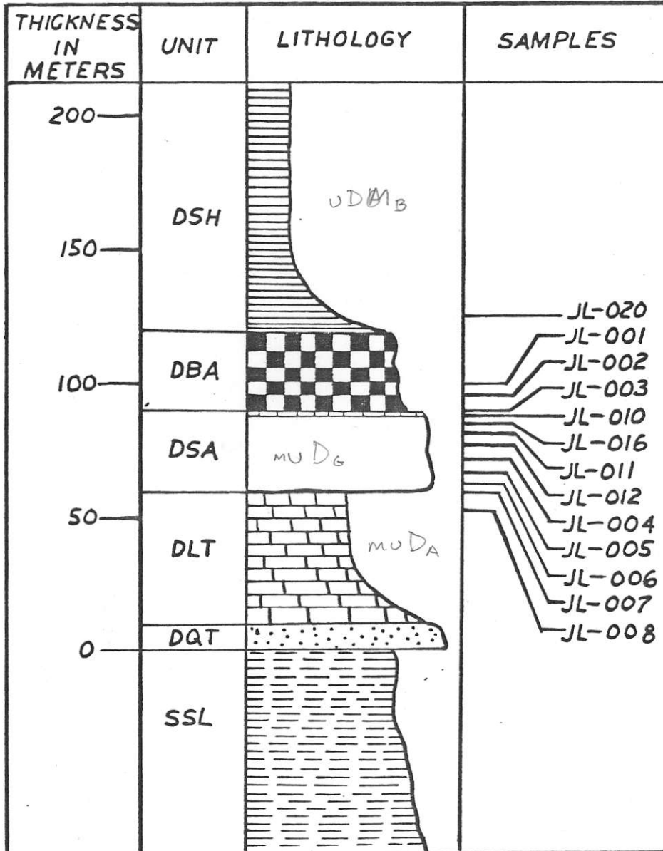
FIGURE 2-7: STRATIGRAPHIC SECTION 1
