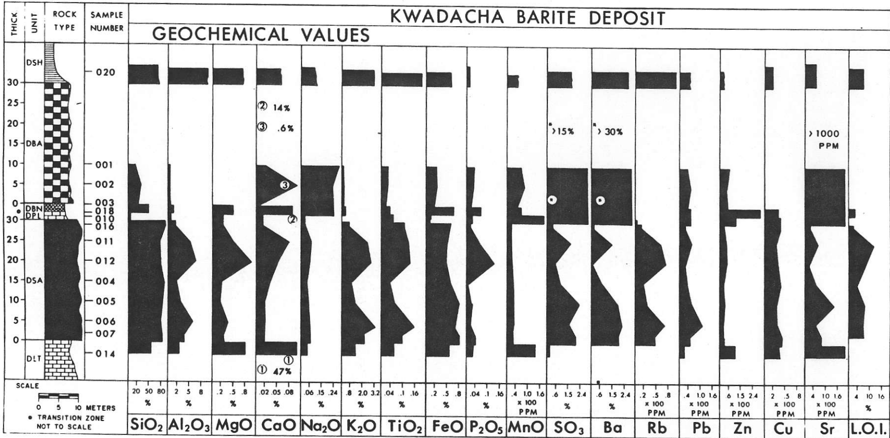
Figure 4-11: Geochemical Stratigraphic Variation at Section 1
