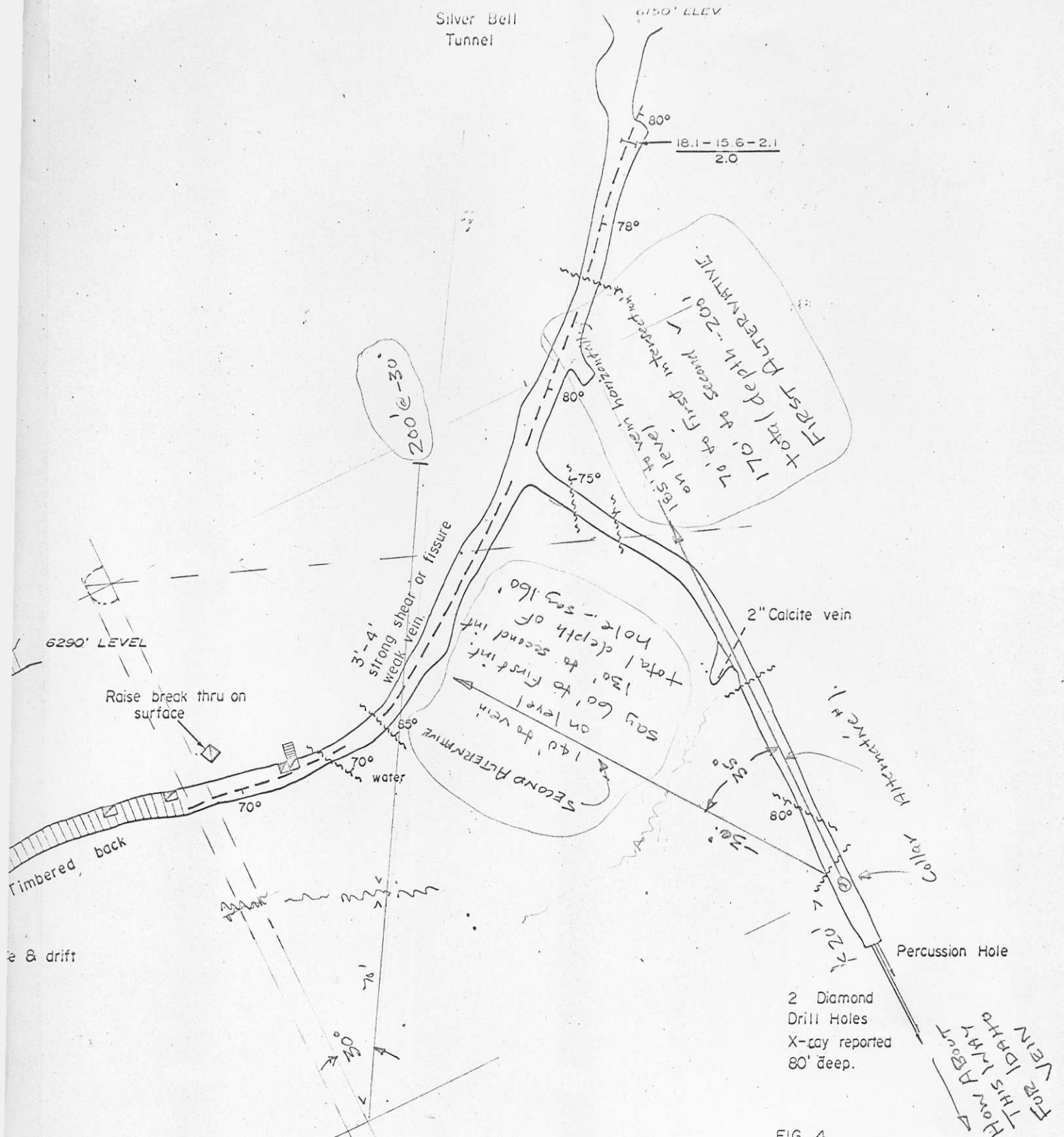
FIG. 4 BACON & CROWHURST LTD. SWIM LAKE MINES LTD. PLAN OF SILVER BELL ADITS & SURFACE CUTS NEW DENVER, B.C.
