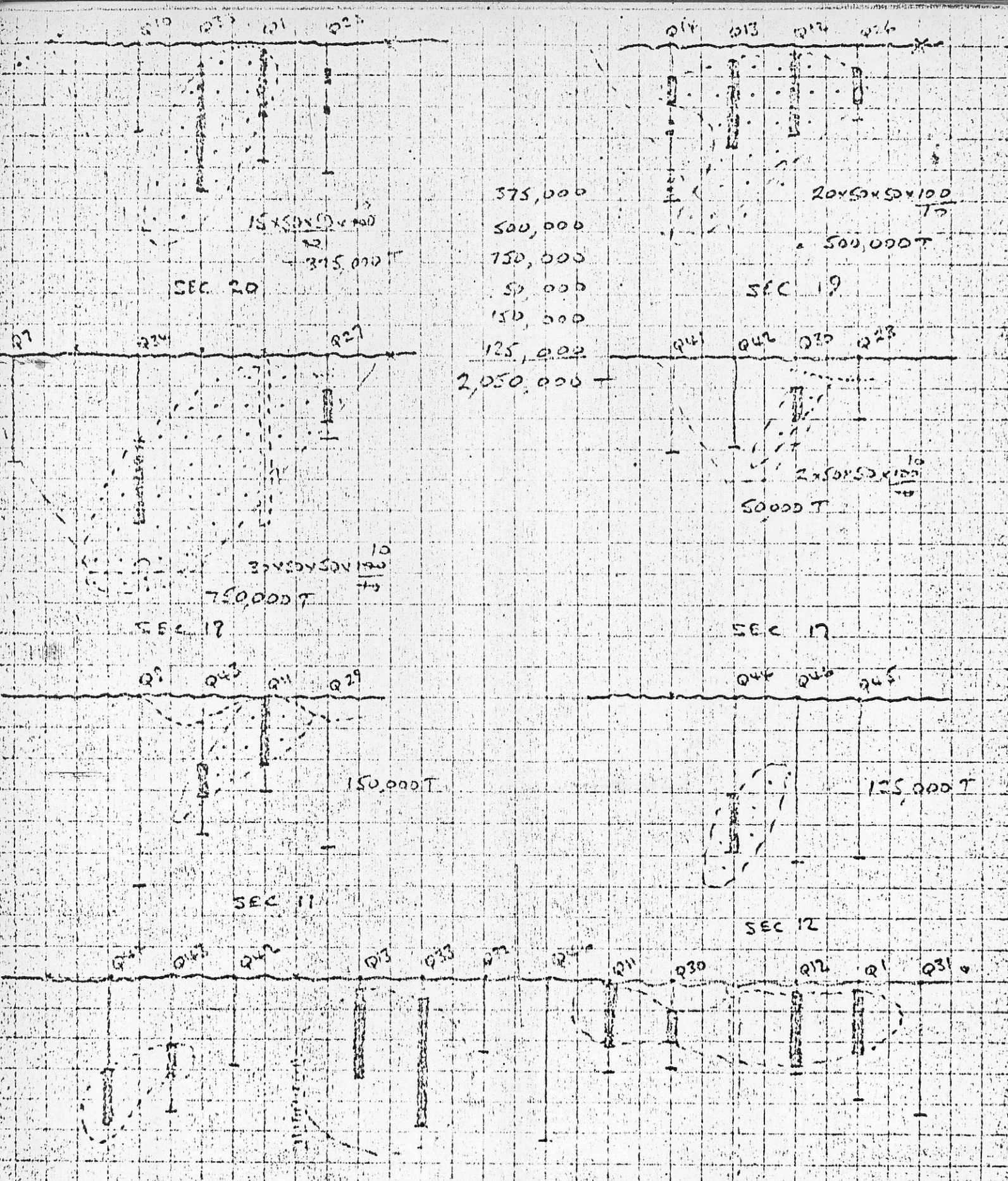
ASTOR MINES - PERCUSSION DRILL SECTIONS WITH TONNAGE ESTIMATE
