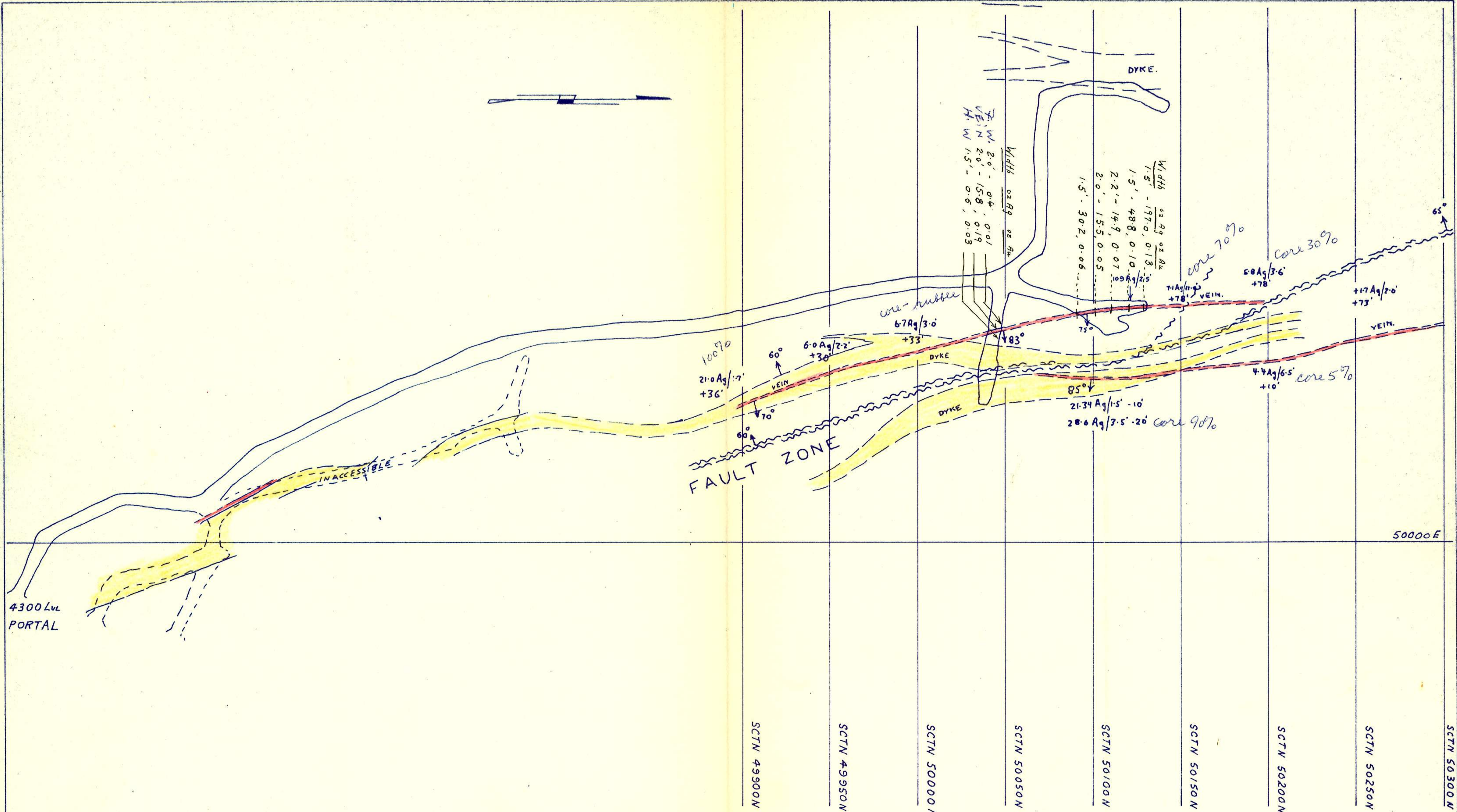
PLAN VIEW - 4300 LEVEL No. 1 ZONE 1" = 50'
