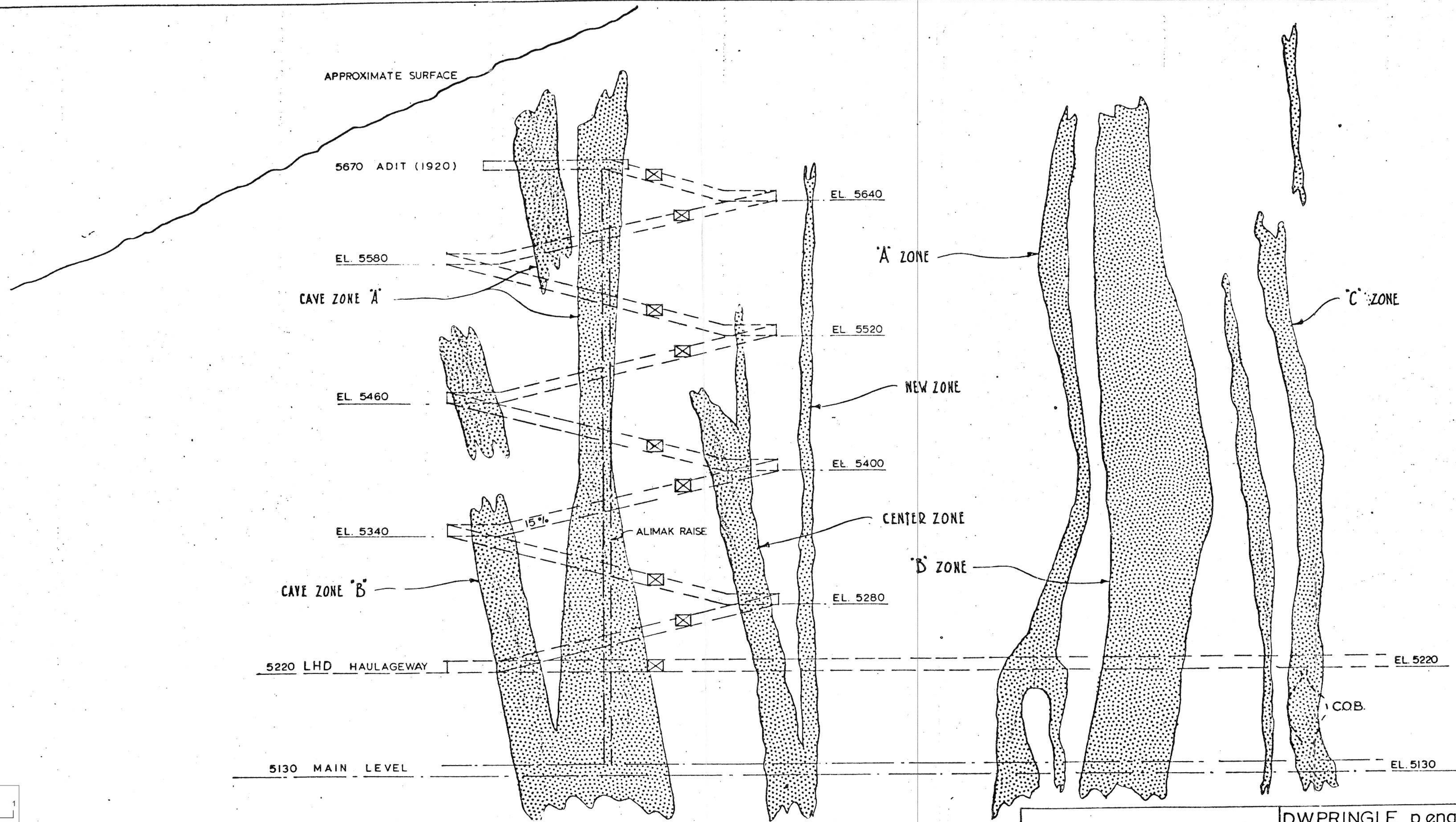
DIAGRAMMATIC SECTION PARALLEL TO MAIN LEVEL SHOWING ORE ZONES AND THE CAVE RAMP SYSTEM.
