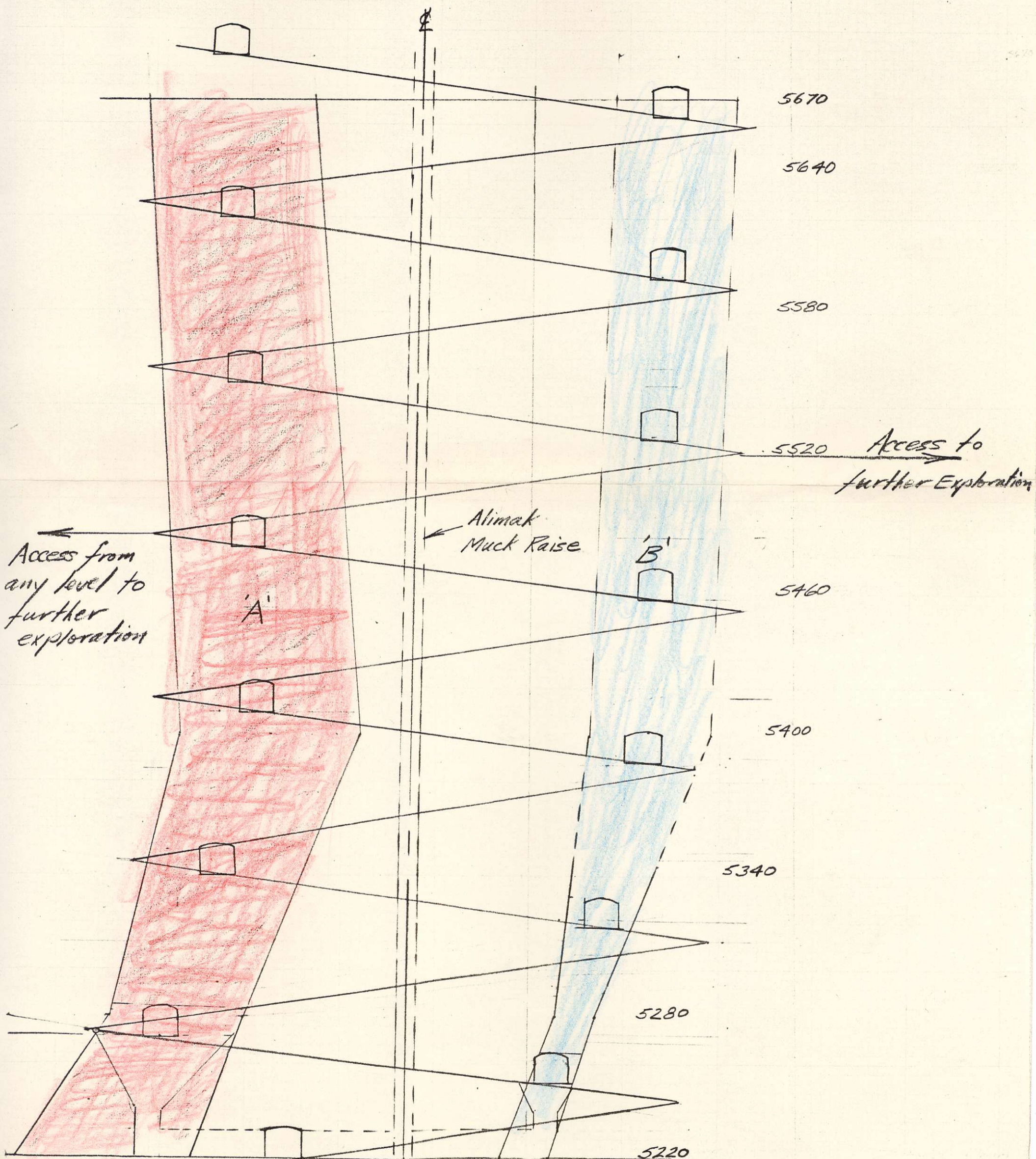
Section Parallel to Main level Scale 1" = 40'
