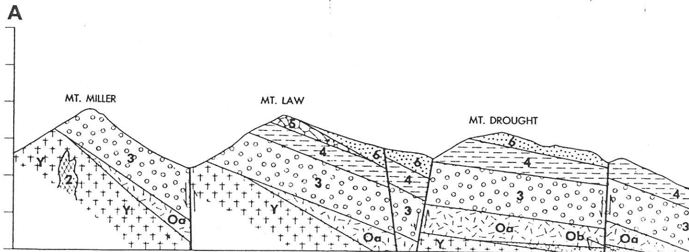
SECTIONAL VIEW MT. MILLER TO WESTBANK, LOOKING NORTHERLY
