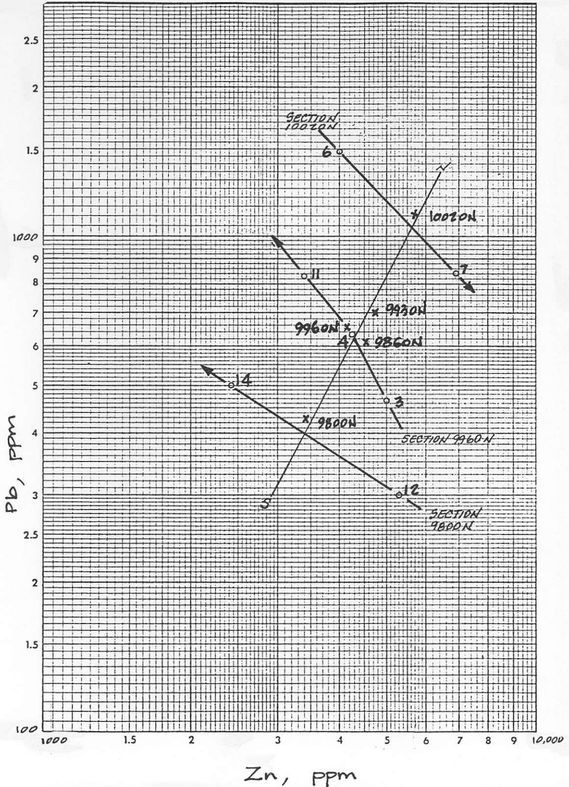
FIGURE 5 - Pb vs. Zn IN DGBP/PR HORIZONS. ARROW HEAD INDICATES DIRECTION OF INCREASING DEPTH. CIRCLES DENOTE DRILL HOLES ON INDIVIDUAL SECTIONS, X'S AVERAGE GRADE FOR EACH SECTION.
