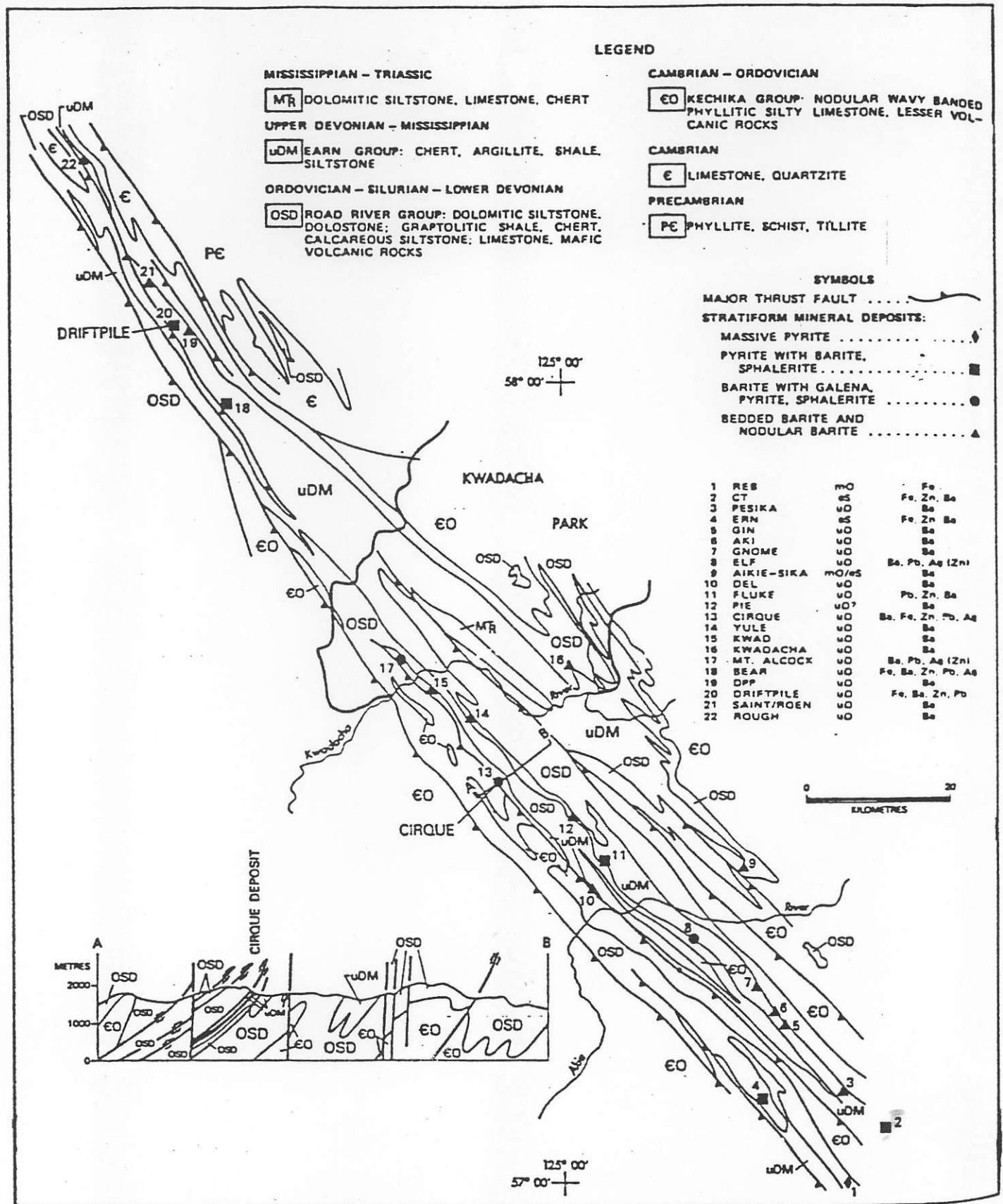
FIGURE 3 - GEOLOGY OF THE GATAGA DISTRICT (McIntyre, 1983).
