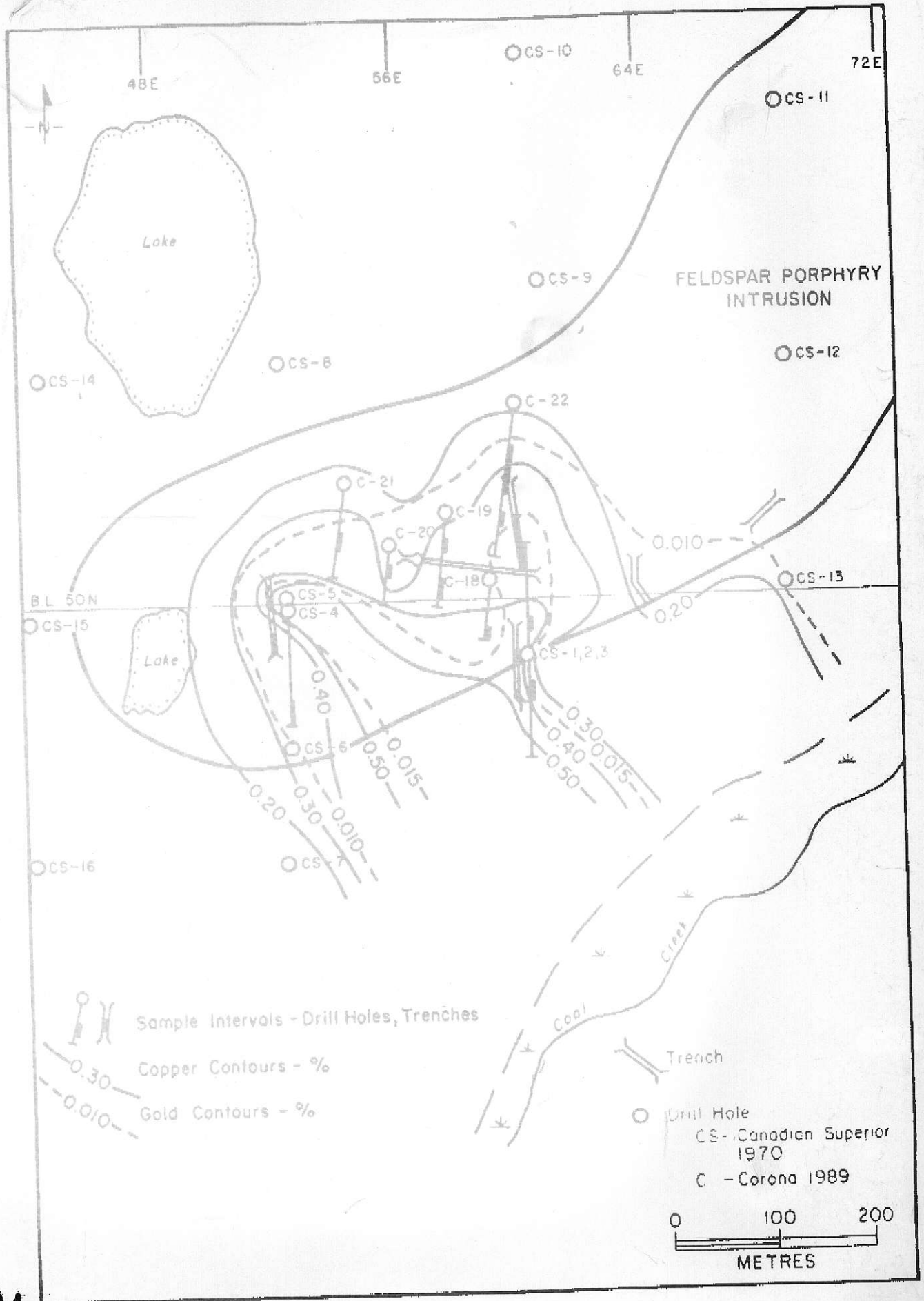
FIGURE 6 - COPPER AND GOLD IN BEDROCK
