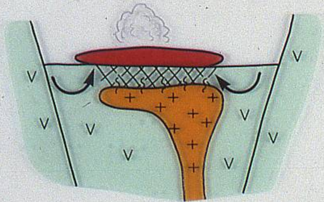
WINDY-CRAGGY Cu-Co (Zn)
