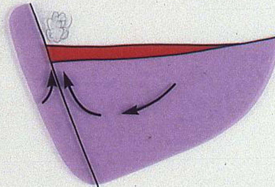
CIRQUE Ba-Zn-Pb-Ag
