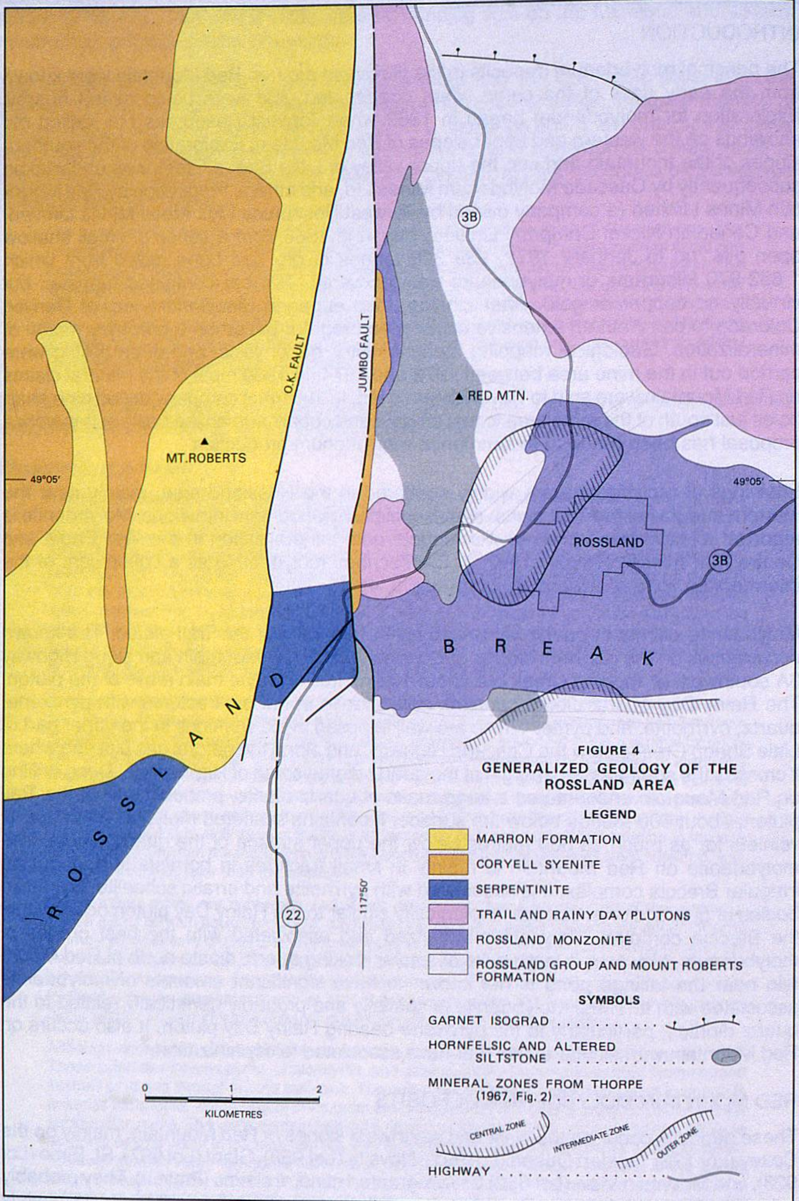
Figure 4. Generalized geology of the Rossland area.
