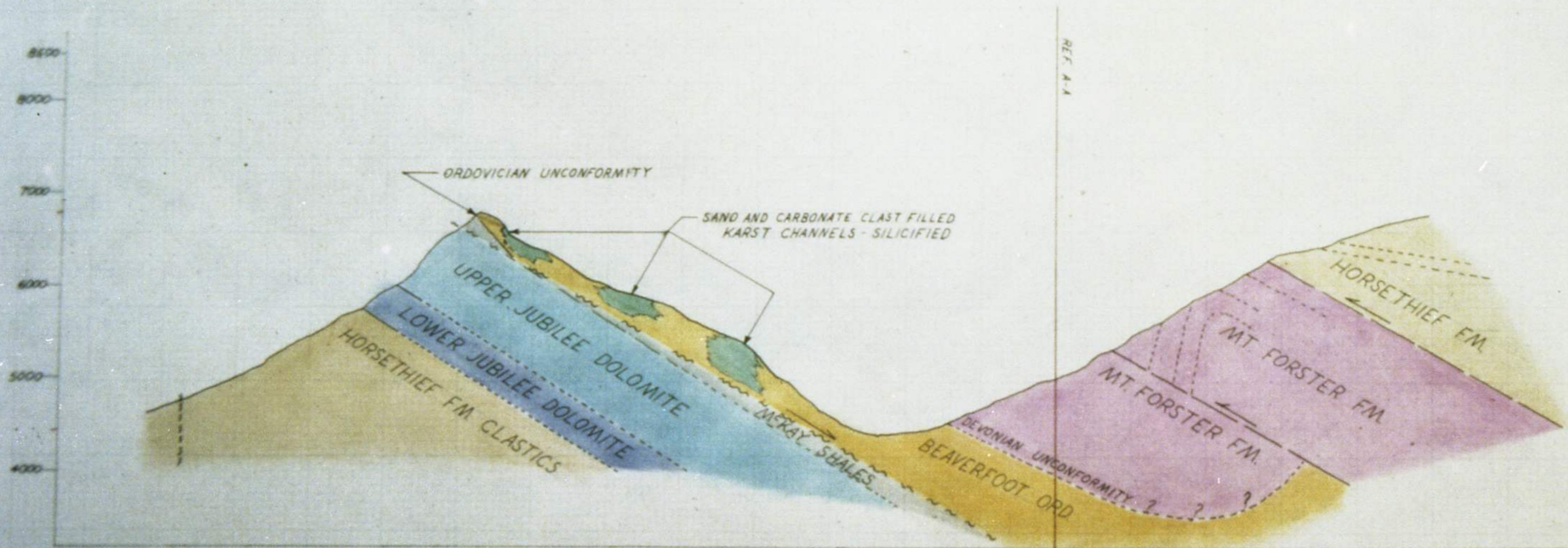
BALTIC SEC A-A 1":800'
