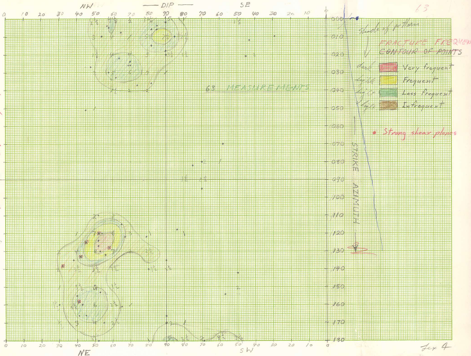
Figure 8 - Lexington Mines Limited, a statistical plot of fractures in the quartz porphyry unit, City of Paris area.
