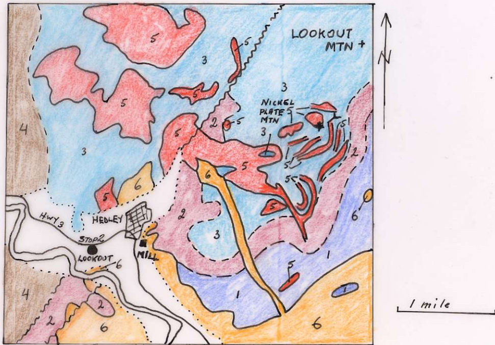
FIG 9:1 GEOLOGY IN THE VICINITY OF HEDLEY ( MODIFIED AFTER BOSTOCK, 1940)
