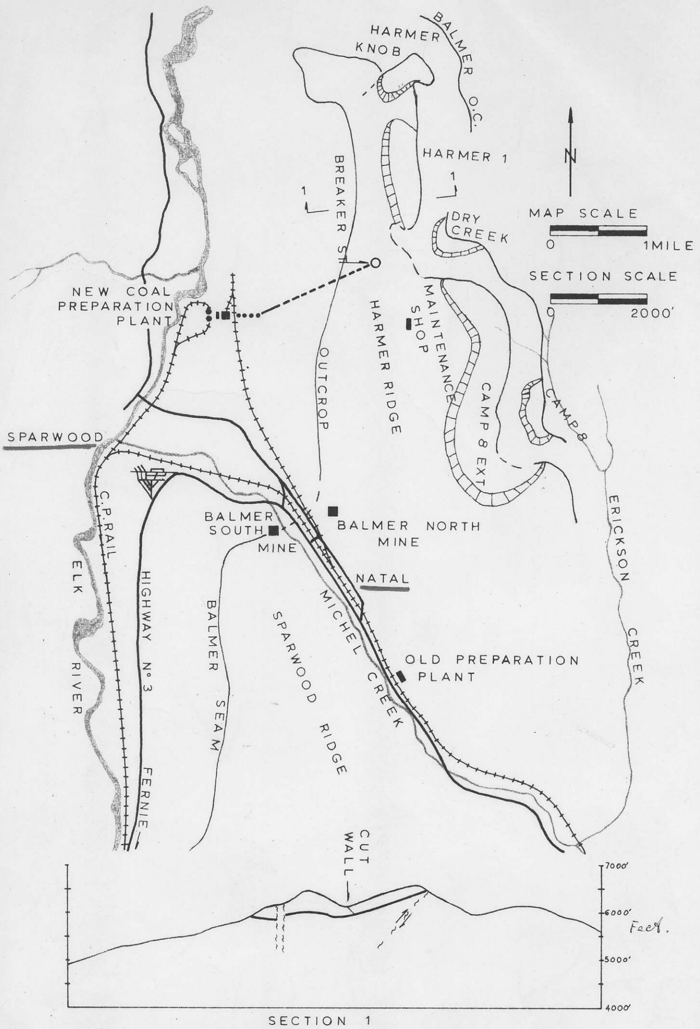
Figure 2:5 : Sketch map of coal mining operations in Fermie Coal Basin
