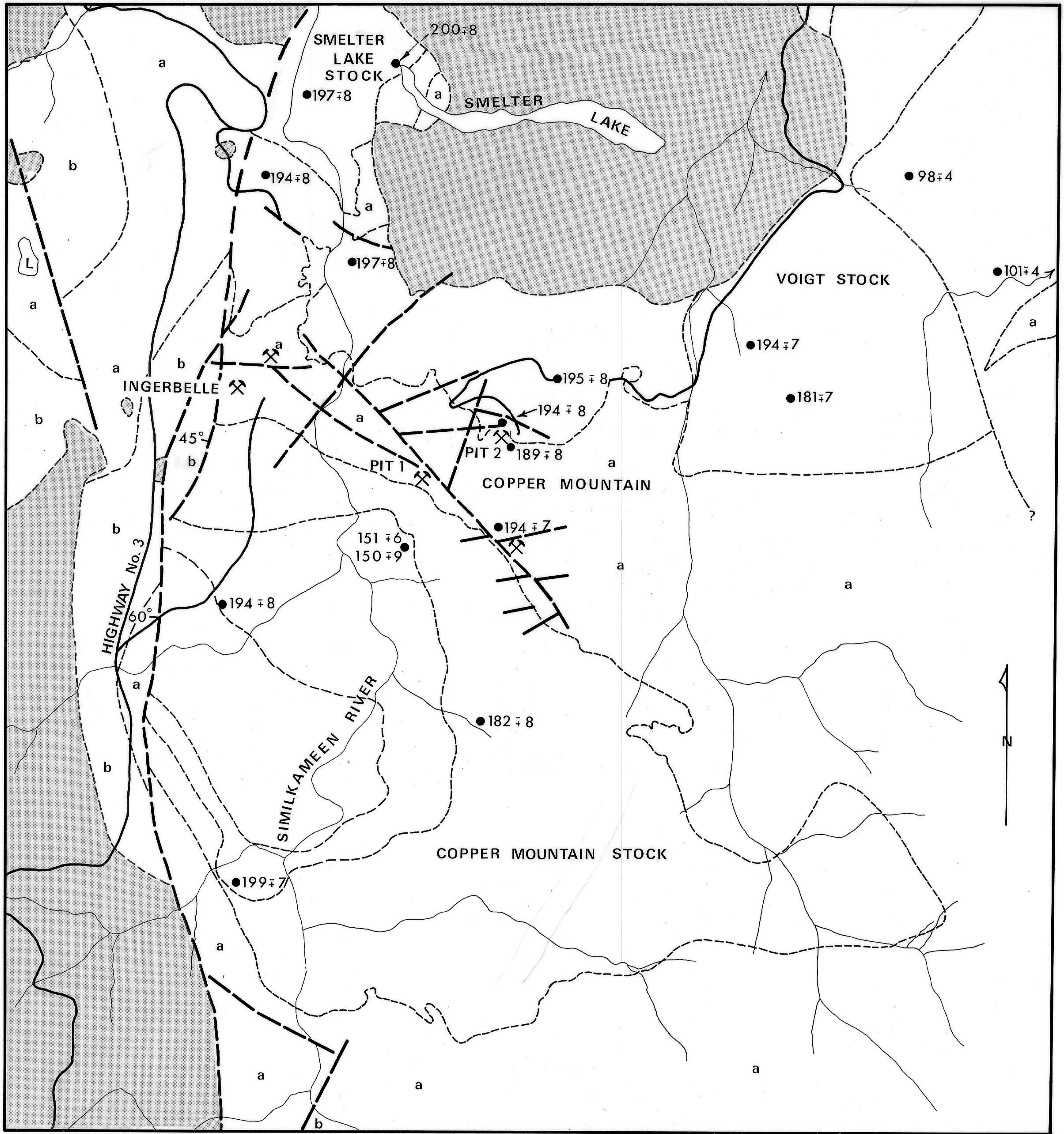
Figure 1 GENERALIZED GEOLOGY OF THE COPPER MOUNTAIN AREA
