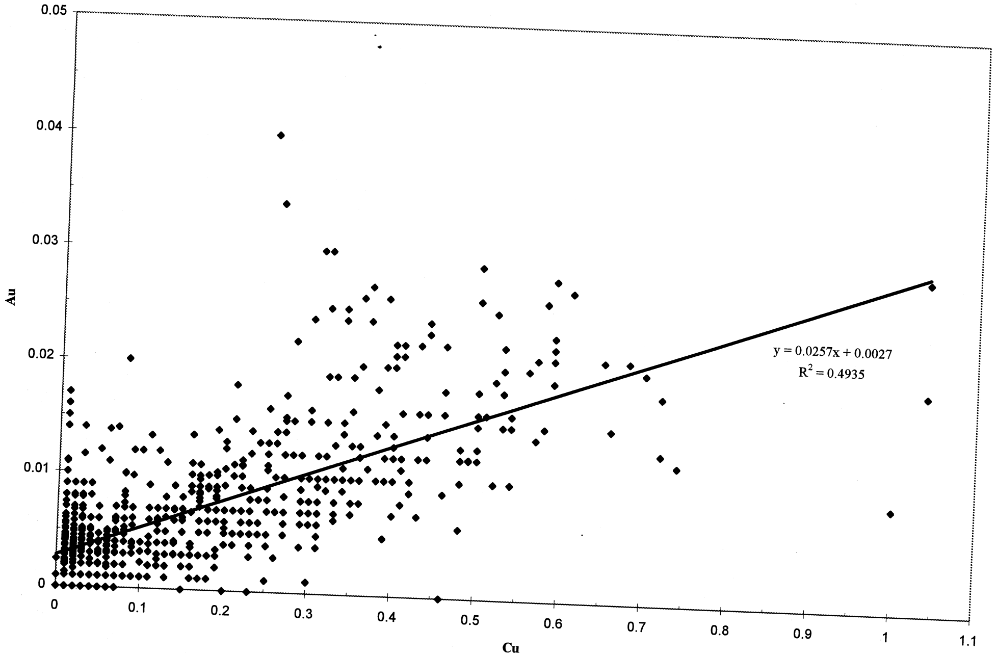
East of Fence1: Au vs. Cu Scatter Plot
