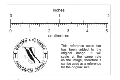
CRAIGMONT DEPOSIT NORANDA AEROMAGNETIC PROFILE No 1 500' TERRAIN CLEARANCE Vertical scale 1" = 100 gammas Horizontal scale 1" = 1320 feet.
