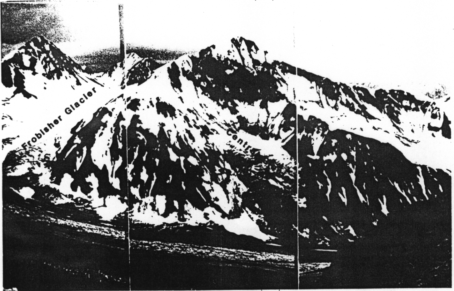
Fig. 3 North Face of Windy Craggy showing the area of sulphide outcrops above the Central Glacier.
