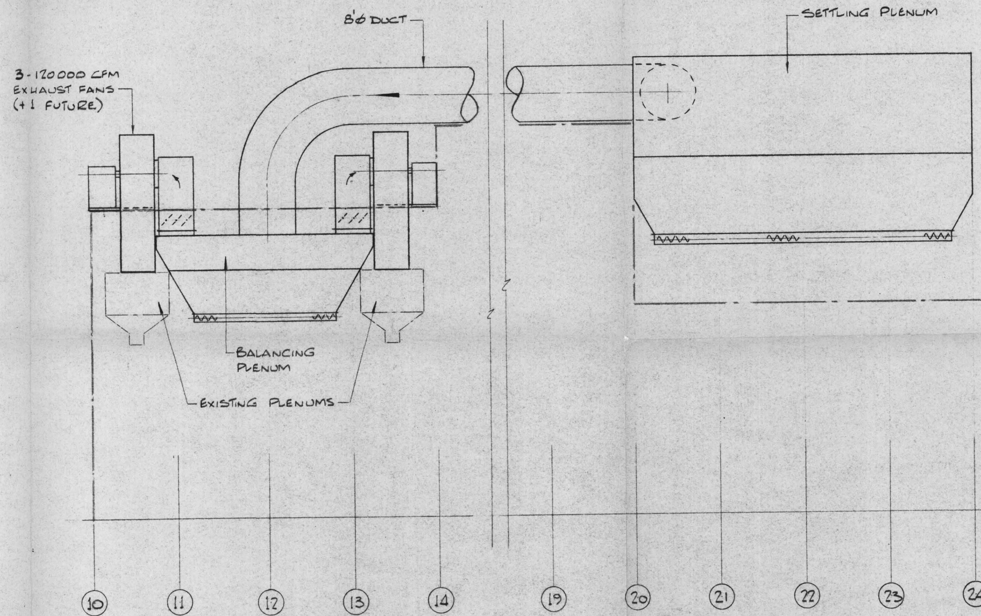
SECTION B-B
