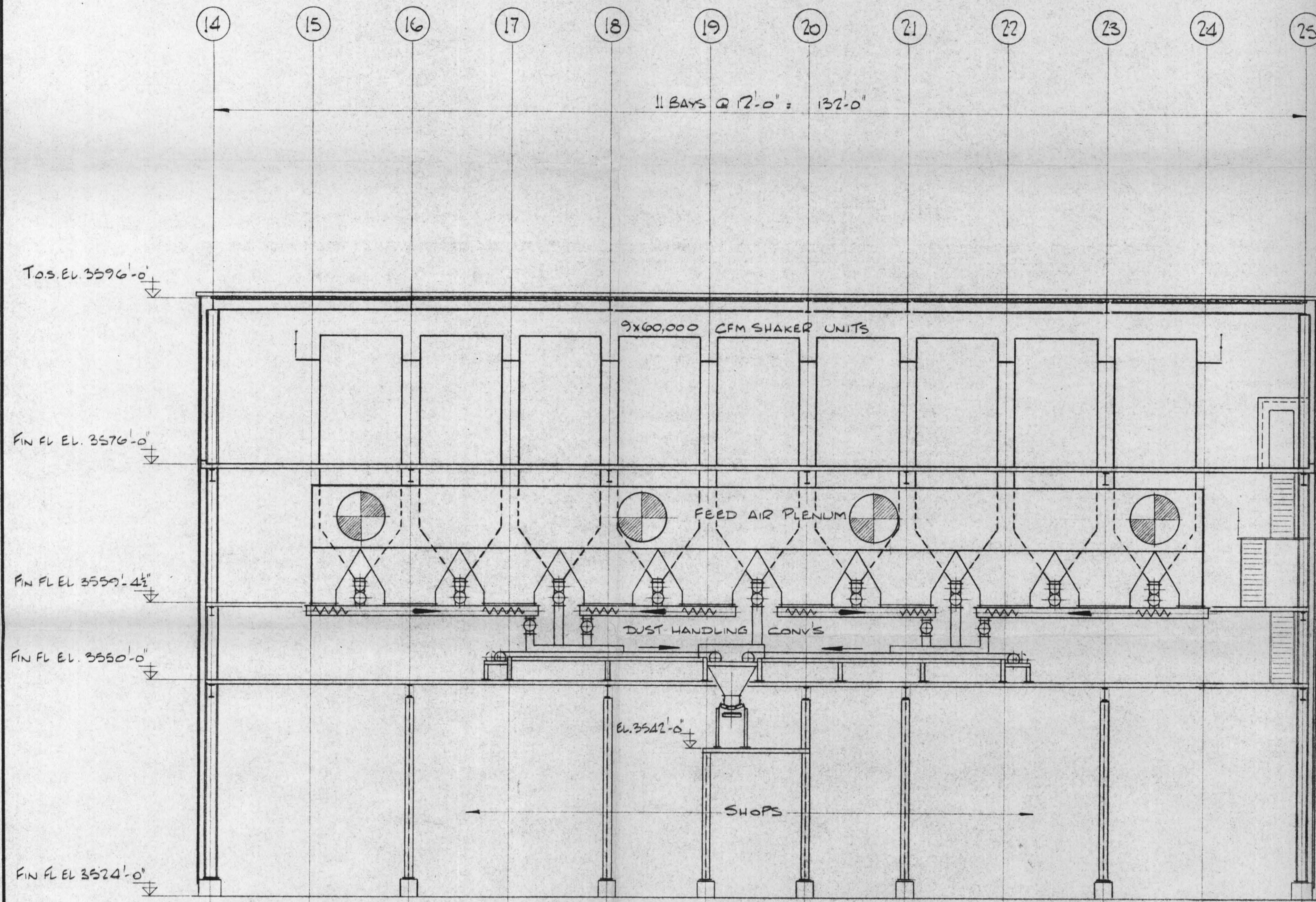
SECTION B-B
