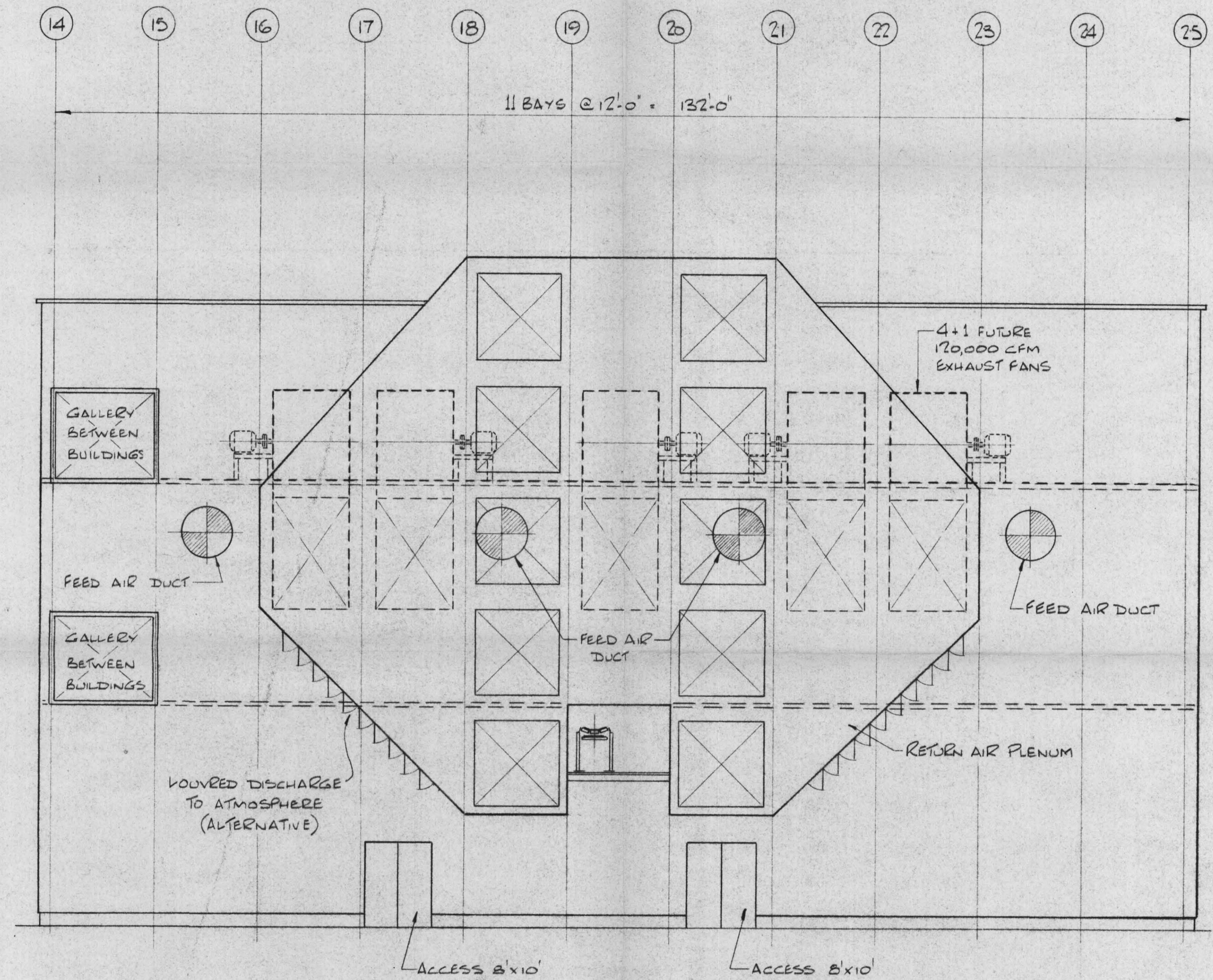
SECTION C-C
