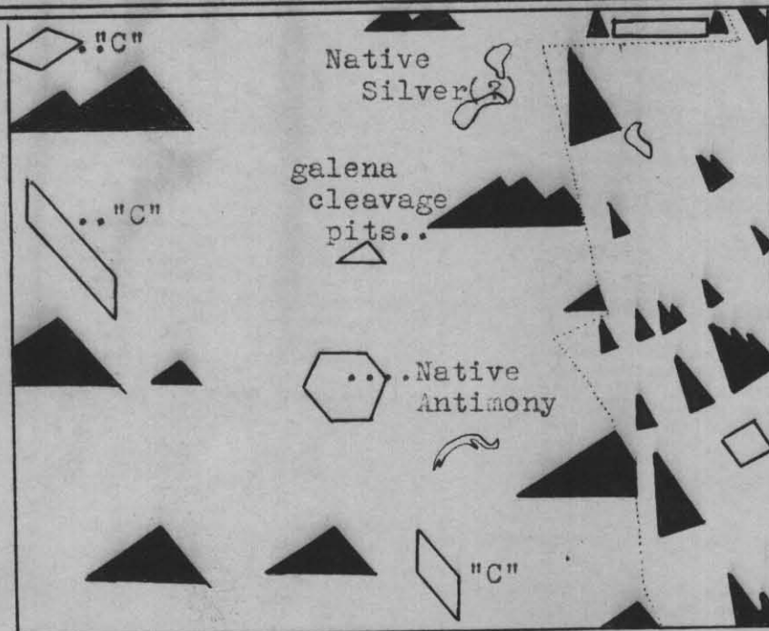
Fig. 8. Preferred Orientation of Unknown "C" (dyscrasite) in Galena.
